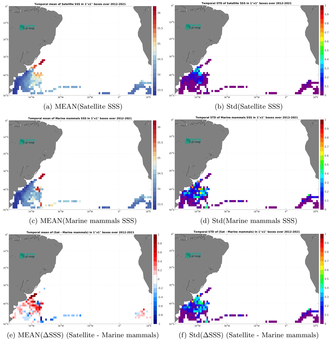
Figure 7: Temporal mean (left) and Std (right) of SSS from SMAP SSS L4 OI v3 - Monthly (ESR) (top), Marine mammals (middle), and of \Delta SSS (Satellite - Marine mammals). Only match-up pairs are used to generate these maps.
