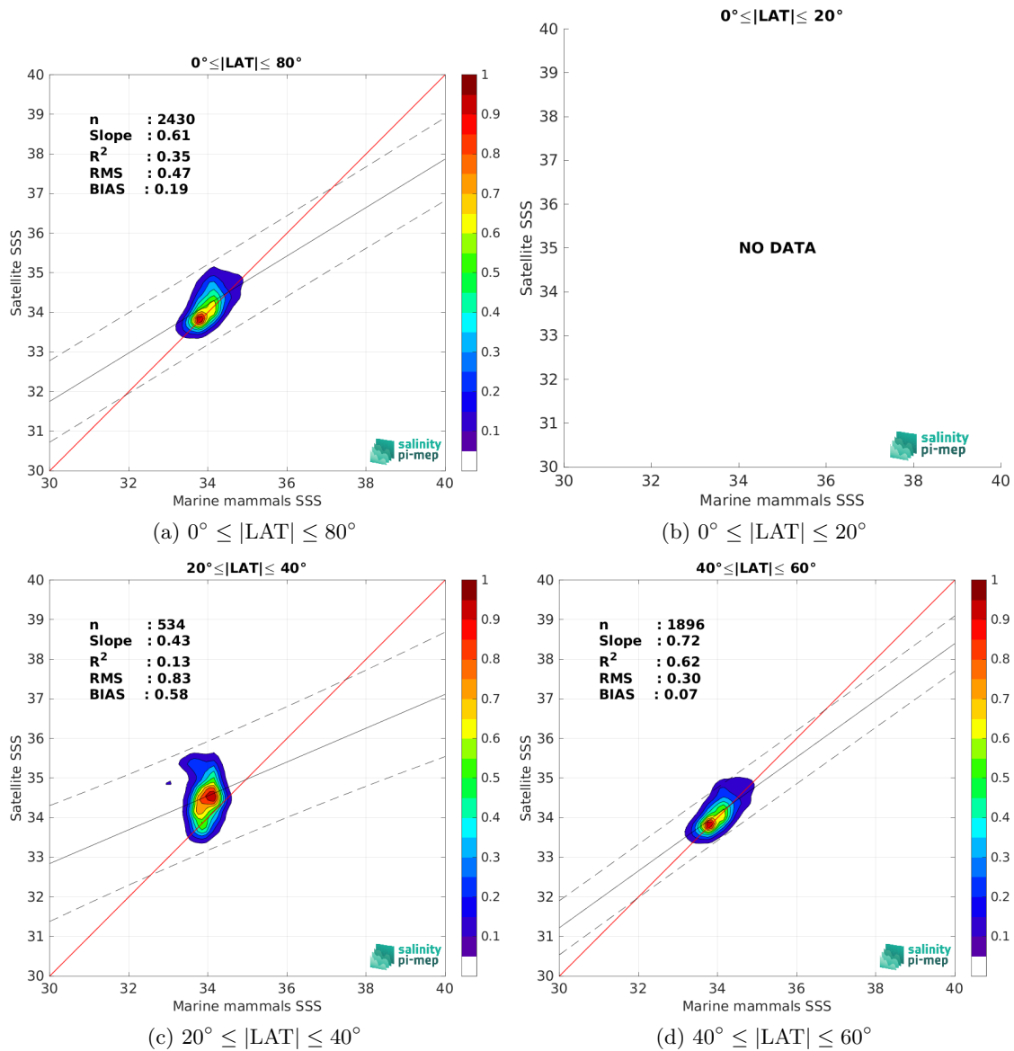
Figure 10: Contour maps of the concentration of SMAP SSS L4 OI v3 - Monthly (ESR) SSS (y-axis) versus Marine mammals SSS (x-axis) at match-up pairs for different latitude bands. For each plot, the red line shows x=y . The black thin and dashed lines indicate a linear fit through the data cloud and the \pm 95\% confidence levels, respectively. The number match-up pairs n , the slope and R^2 coefficient of the linear fit, the root mean square (RMS) and the mean bias between satellite and in situ data are indicated for each latitude band in each plots.
