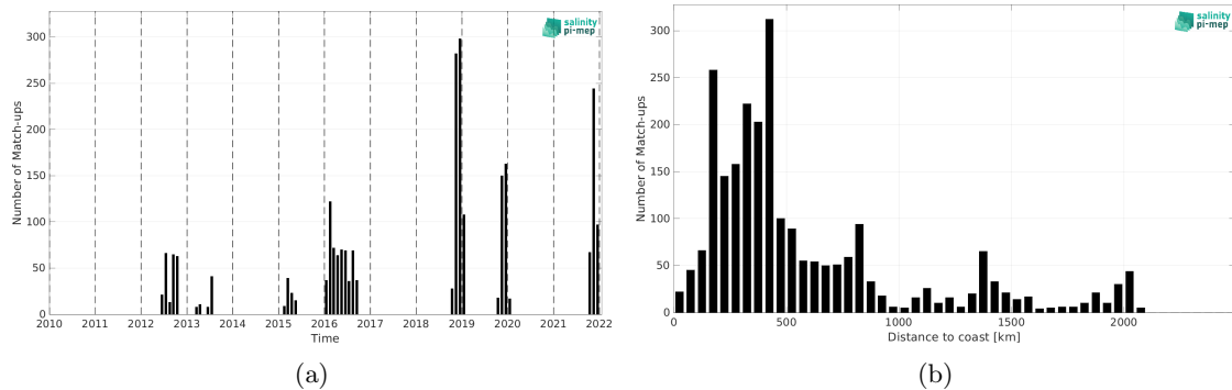
Figure 2: Number of match-ups between Marine mammals and SMAP SSS L4 OI v3 - Monthly (ESR) SSS as a function of time (a) and as function of the distance to coast (b) over the South Atlantic Ocean Pi-MEP region and for the full satellite product period.
