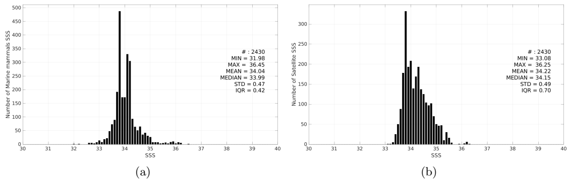
Figure 3: Histograms of SSS from Marine mammals (a) and SMAP SSS L4 OI v3 - Monthly (ESR) (b) considering all match-up pairs per bins of 0.1 over the South Atlantic Ocean Pi-MEP region and for the full satellite product period.
