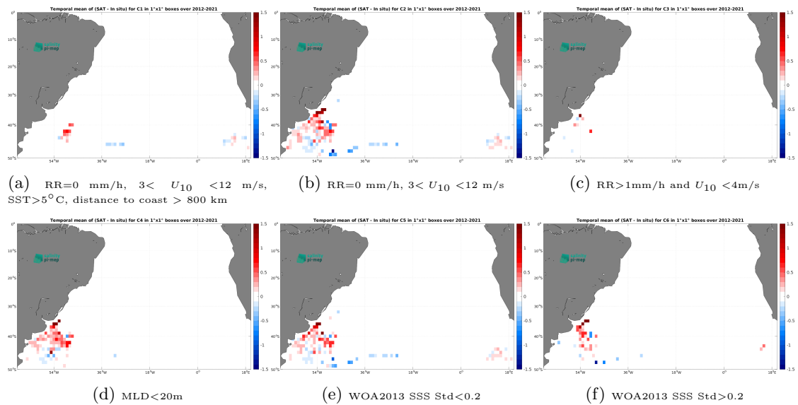
Figure 14: Temporal mean gridded over spatial boxes of size 1^\circ \times 1^\circ of \Delta SSS (SMAP SSS L4 OI v3 - Monthly (ESR) - Marine mammals) for 6 different subdatasets corresponding to:RR=0 mm/h, 3 < U_{10} < 12 m/s, SST >5^\circ C, distance to coast > 800 km (a), RR=0 mm/h, 3 < U_{10} < 12 m/s (b), RR >1 mm/h and U_{10} < 4 m/s (c),MLD <20 m (d),WOA2013 SSS Std <0.2 (e),WOA2013 SSS Std >0.2 (f).
