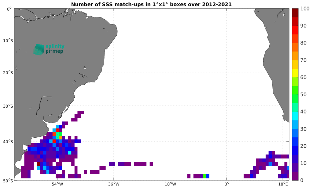
Figure 5: Number of SSS match-ups between Marine mammals SSS and the SMAP SSS L4 OI v3 - Monthly (ESR) SSS product for the South Atlantic Ocean Pi-MEP region over 1^\circ \times 1^\circ boxes and for the full satellite product period.
