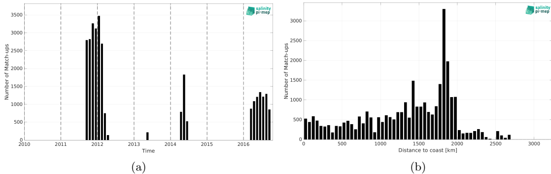
Figure 2: Number of match-ups between Surface drifters and SMAP SSS L4 OI v3 - Monthly (ESR) SSS as a function of time (a) and as function of the distance to coast (b) over the South Atlantic Ocean Pi-MEP region and for the full satellite product period.
