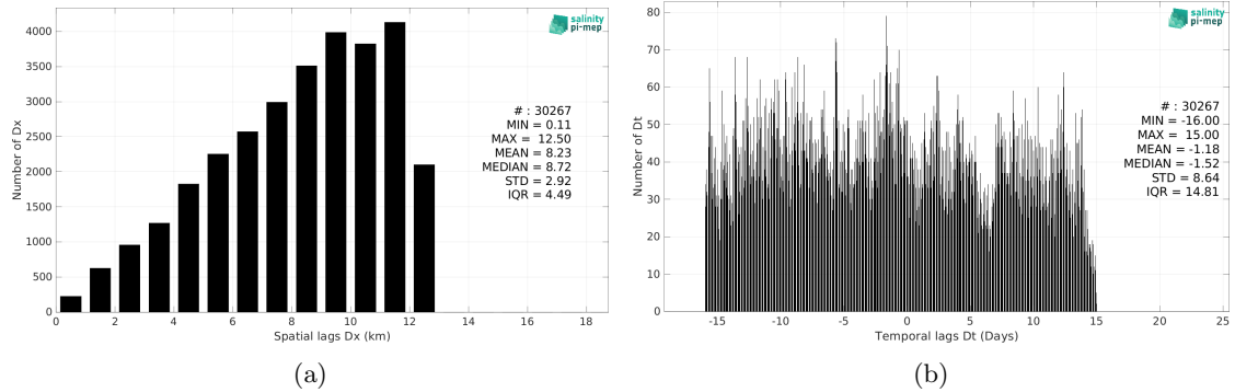
Figure 5: Histograms of the spatial (a) and temporal (b) lags between the location/time of the Surface drifters measurement and the date of the corresponding SMAP SSS L4 OI v3 - Monthly (ESR) SSS pixel.
