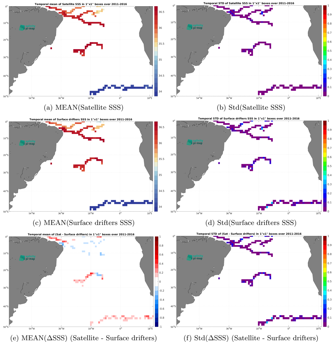
Figure 6: Temporal mean (left) and Std (right) of SSS from SMAP SSS L4 OI v3 - Monthly (ESR) (top), Surface drifters (middle), and of \Delta SSS (Satellite - Surface drifters). Only match-up pairs are used to generate these maps.
