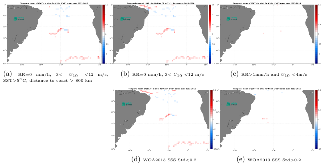
Figure 13: Temporal mean gridded over spatial boxes of size 1^\circ \times 1^\circ of \Delta SSS (SMAP SSS L4 OI v3 - Monthly (ESR) - Surface drifters) for 5 different subdatasets corresponding to:RR=0 mm/h, 3 < U_{10} < 12 m/s, SST >5^\circ\text{C} , distance to coast > 800 km (a), RR=0 mm/h, 3 < U_{10} < 12 m/s (b), RR >1 mm/h and U_{10} < 4 m/s (c), WOA2013 SSS Std <0.2 (d), WOA2013 SSS Std >0.2 (e).
