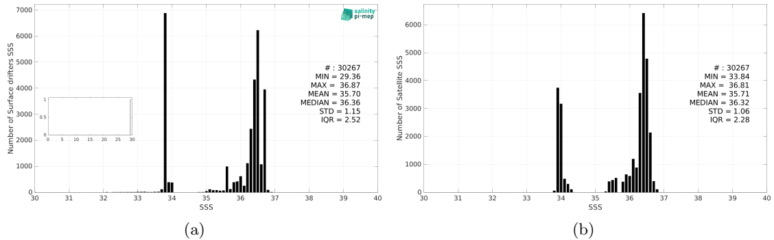
Figure 3: Histograms of SSS from Surface drifters (a) and SMAP SSS L4 OI v3 - Monthly (ESR) (b) considering all match-up pairs per bins of 0.1 over the South Atlantic Ocean Pi-MEP region and for the full satellite product period.
