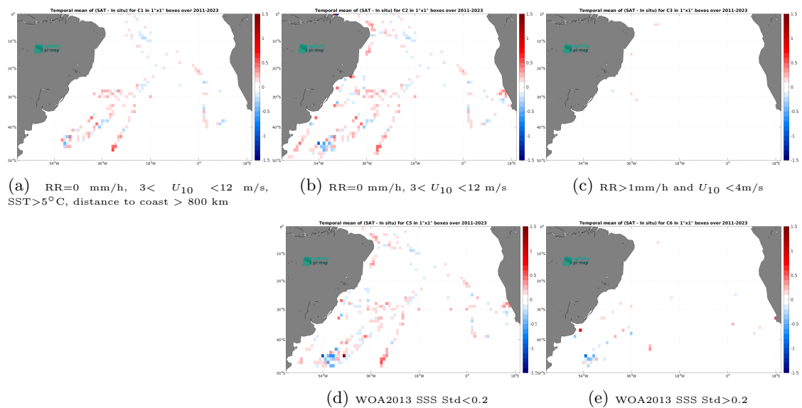
Figure 14: Temporal mean gridded over spatial boxes of size 1^\circ \times 1^\circ of \Delta\text{SSS} (SMAP SSS L4 OI v3 - Daily (ESR) - TSG (SAMOS)) for 5 different subdatasets corresponding to:RR=0 mm/h, 3 < U_{10} < 12 m/s, SST>5°C, distance to coast > 800 km (a), RR=0 mm/h, 3 < U_{10} < 12 m/s (b), RR>1mm/h and U_{10} < 4 m/s (c), WOA2013 SSS Std<0.2 (d), WOA2013 SSS Std>0.2 (e).
