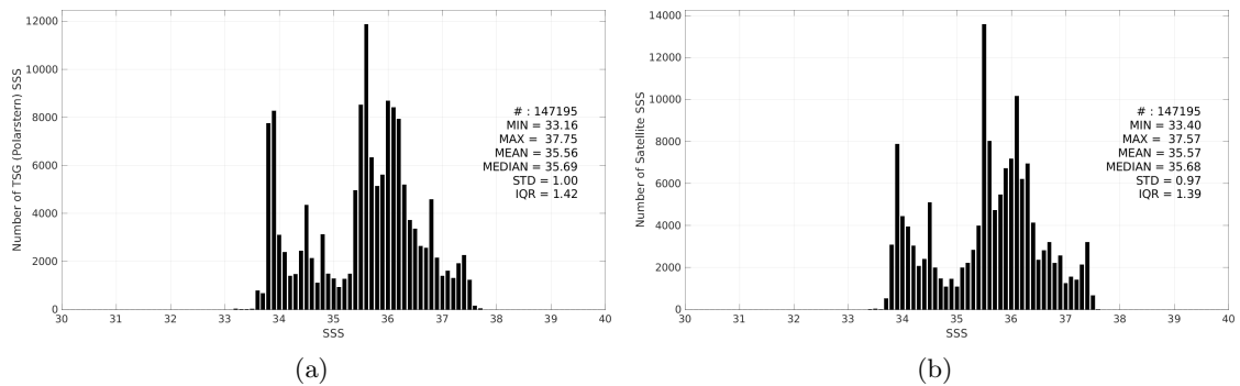
Figure 3: Histograms of SSS from TSG (Polarstern) (a) and SMAP SSS L4 OI v3 - Daily (ESR) (b) considering all match-up pairs per bins of 0.1 over the South Atlantic Ocean Pi-MEP region and for the full satellite product period.
