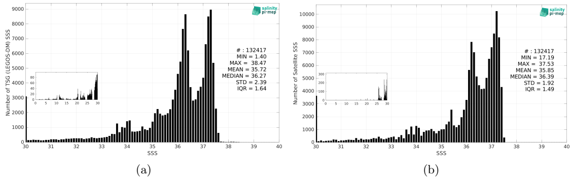
Figure 3: Histograms of SSS from TSG (LEGOS-DM) (a) and SMAP SSS L4 OI v3 - Daily (ESR) (b) considering all match-up pairs per bins of 0.1 over the South Atlantic Ocean Pi-MEP region and for the full satellite product period.
