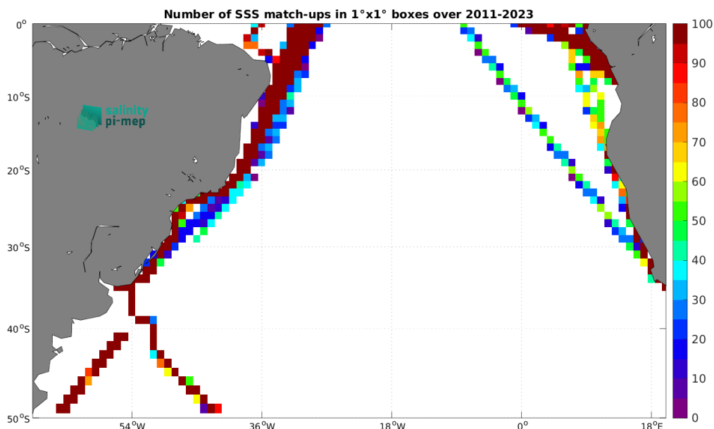
Figure 5: Number of SSS match-ups between TSG (LEGOS-DM) SSS and the SMAP SSS L4 OI v3 - Daily (ESR) SSS product for the South Atlantic Ocean Pi-MEP region over 1^\circ \times 1^\circ boxes and for the full satellite product period.
