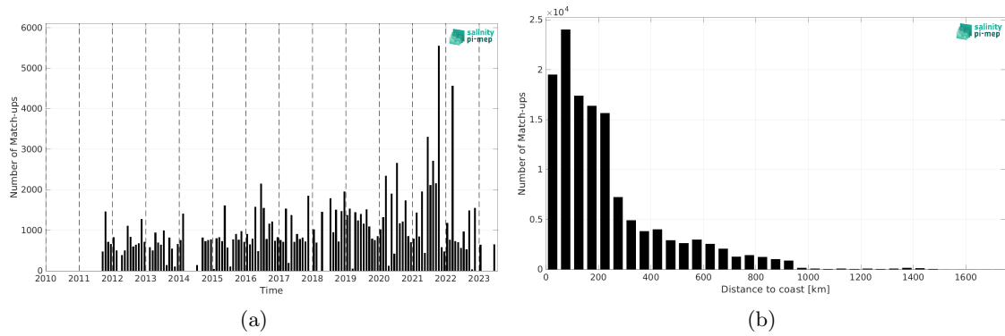
Figure 2: Number of match-ups between TSG (LEGOS-DM) and SMAP SSS L4 OI v3 - Daily (ESR) SSS as a function of time (a) and as function of the distance to coast (b) over the South Atlantic Ocean Pi-MEP region and for the full satellite product period.
