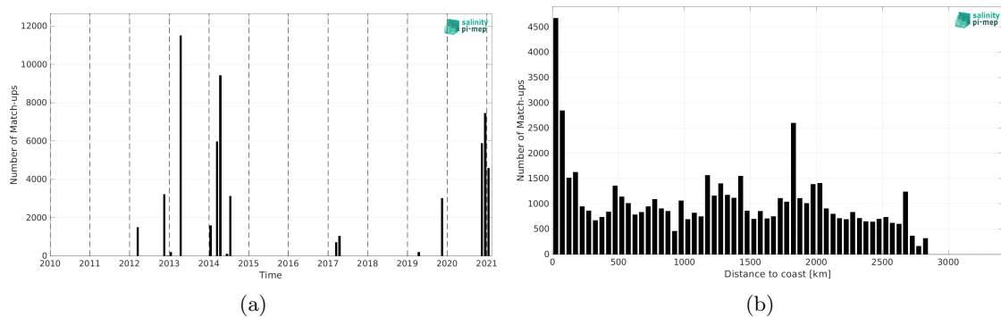
Figure 2: Number of match-ups between TSG (GOSUD-Sailing-ship) and SMAP SSS L4 OI v3 - Daily (ESR) SSS as a function of time (a) and as function of the distance to coast (b) over the South Atlantic Ocean Pi-MEP region and for the full satellite product period.
