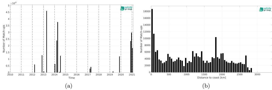
Figure 2: Number of match-ups between TSG (GOSUD-Sailing-ship) and SMAP SSS L4 OI v3 - Daily (ESR) SSS as a function of time (a) and as function of the distance to coast (b) over the South Atlantic Ocean Pi-MEP region and for the full satellite product period.
