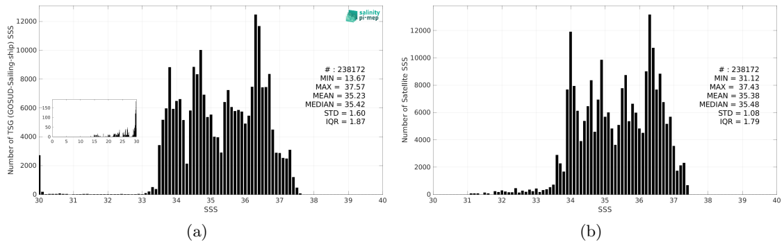
Figure 3: Histograms of SSS from TSG (GOSUD-Sailing-ship) (a) and SMAP SSS L4 OI v3 - Daily (ESR) (b) considering all match-up pairs per bins of 0.1 over the South Atlantic Ocean Pi-MEP region and for the full satellite product period.
