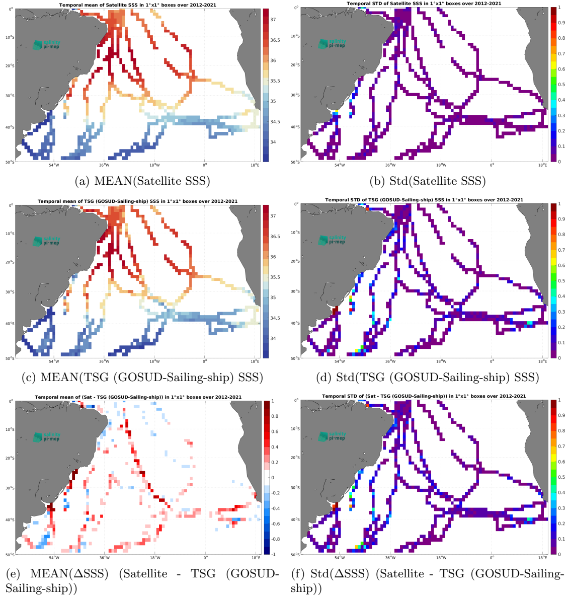
Figure 7: Temporal mean (left) and Std (right) of SSS from SMAP SSS L4 OI v3 - Daily (ESR) (top), TSG (GOSUD-Sailing-ship) (middle), and of \Delta SSS (Satellite - TSG (GOSUD-Sailing-ship)). Only match-up pairs are used to generate these maps.
