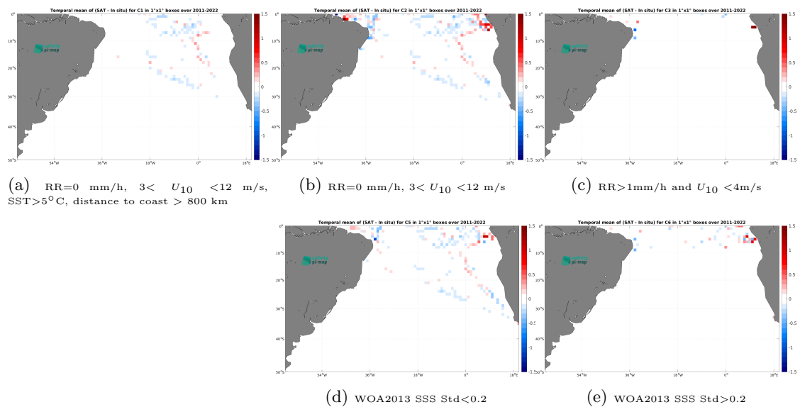
Figure 14: Temporal mean gridded over spatial boxes of size 1^\circ \times 1^\circ of \Delta SSS (SMAP SSS L4 OI v3 - Daily (ESR) - TSG (GOSUD-Research-vessel)) for 5 different subdatasets corresponding to:RR=0 mm/h, 3 < U_{10} < 12 m/s, SST >5^\circ C, distance to coast > 800 km (a), RR=0 mm/h, 3 < U_{10} < 12 m/s (b), RR >1 mm/h and U_{10} < 4 m/s (c), WOA2013 SSS Std <0.2 (d), WOA2013 SSS Std >0.2 (e).
