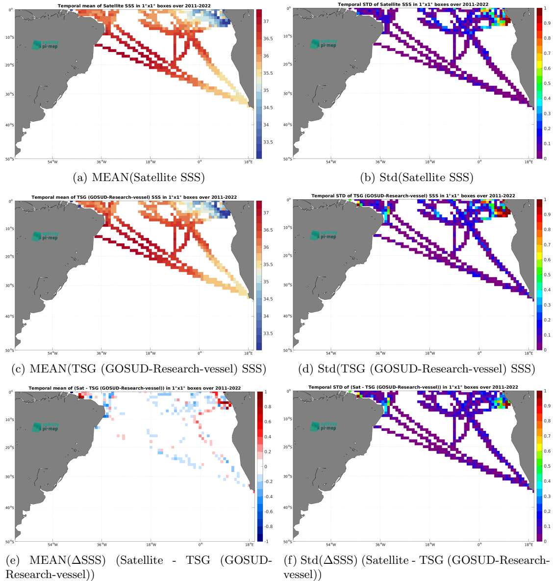
Figure 7: Temporal mean (left) and Std (right) of SSS from SMAP SSS L4 OI v3 - Daily (ESR) (top), TSG (GOSUD-Research-vessel) (middle), and of \Delta SSS (Satellite - TSG (GOSUD-Research-vessel)). Only match-up pairs are used to generate these maps.
