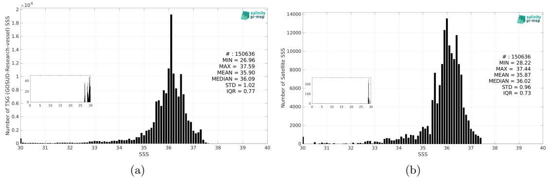
Figure 3: Histograms of SSS from TSG (GOSUD-Research-vessel) (a) and SMAP SSS L4 OI v3 - Daily (ESR) (b) considering all match-up pairs per bins of 0.1 over the South Atlantic Ocean Pi-MEP region and for the full satellite product period.
