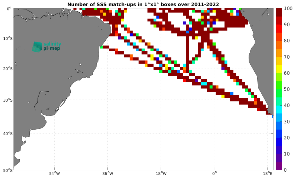
Figure 5: Number of SSS match-ups between TSG (GOSUD-Research-vessel) SSS and the SMAP SSS L4 OI v3 - Daily (ESR) SSS product for the South Atlantic Ocean Pi-MEP region over 1^\circ \times 1^\circ boxes and for the full satellite product period.
