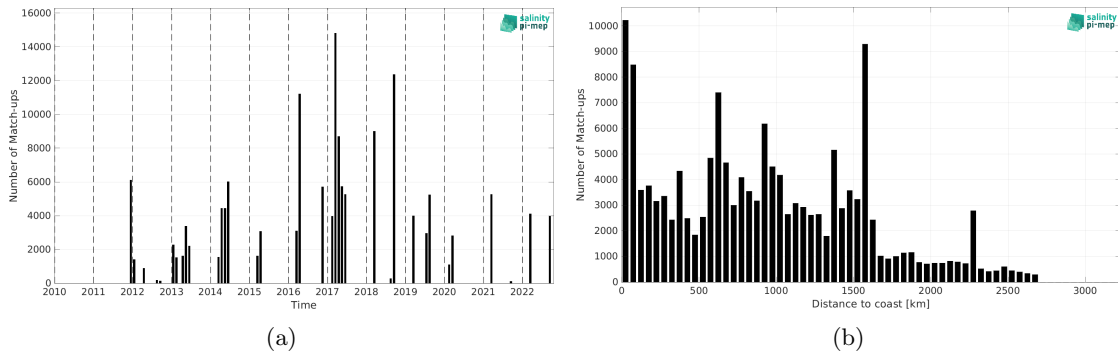
Figure 2: Number of match-ups between TSG (GOSUD-Research-vessel) and SMAP SSS L4 OI v3 - Daily (ESR) SSS as a function of time (a) and as function of the distance to coast (b) over the South Atlantic Ocean Pi-MEP region and for the full satellite product period.
