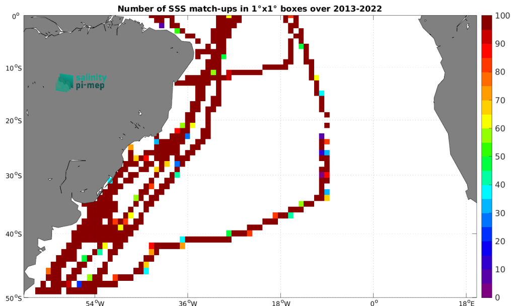
Figure 5: Number of SSS match-ups between TSG (CSIC-UTM) SSS and the SMAP SSS L4 OI v3 - Daily (ESR) SSS product for the South Atlantic Ocean Pi-MEP region over 1^\circ \times 1^\circ boxes and for the full satellite product period.
