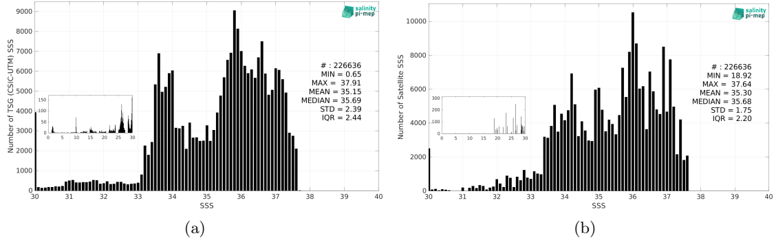
Figure 3: Histograms of SSS from TSG (CSIC-UTM) (a) and SMAP SSS L4 OI v3 - Daily (ESR) (b) considering all match-up pairs per bins of 0.1 over the South Atlantic Ocean Pi-MEP region and for the full satellite product period.
