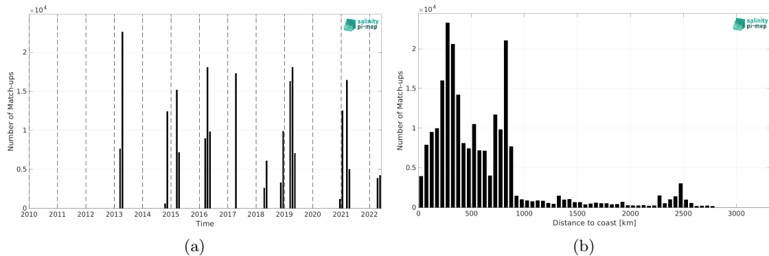
Figure 2: Number of match-ups between TSG (CSIC-UTM) and SMAP SSS L4 OI v3 - Daily (ESR) SSS as a function of time (a) and as function of the distance to coast (b) over the South Atlantic Ocean Pi-MEP region and for the full satellite product period.
