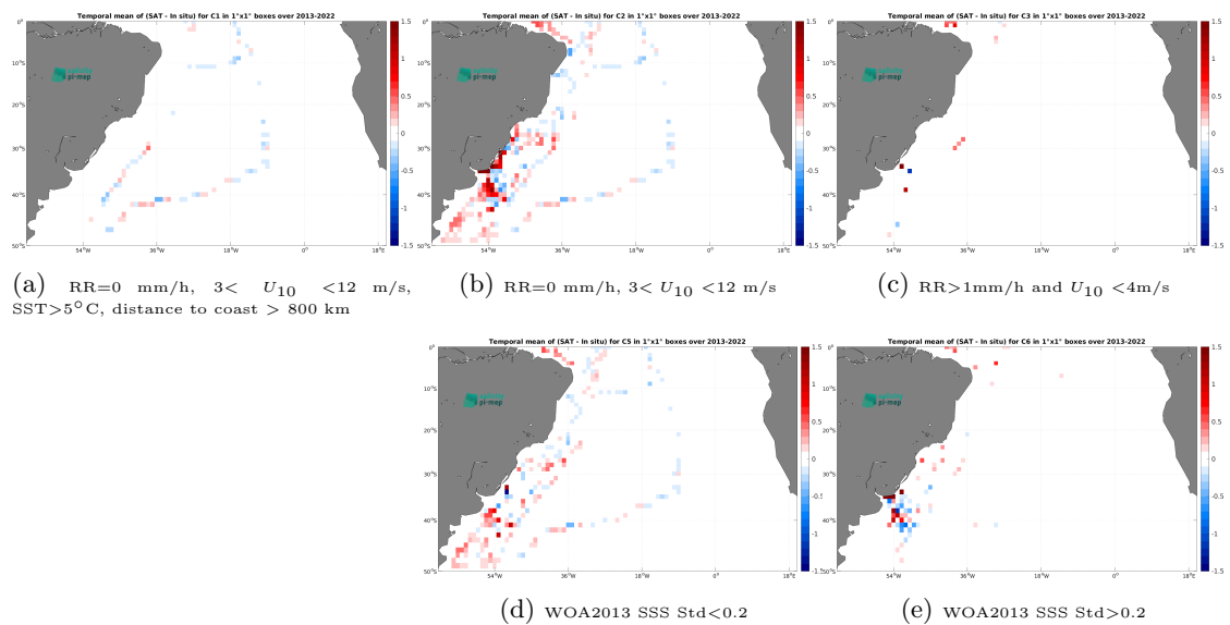
Figure 14: Temporal mean gridded over spatial boxes of size 1^\circ \times 1^\circ of \Delta SSS (SMAP SSS L4 OI v3 - Daily (ESR) - TSG (CSIC-UTM)) for 5 different subdatasets corresponding to:RR=0 mm/h, 3 < U_{10} < 12 m/s, SST > 5°C, distance to coast > 800 km (a), RR=0 mm/h, 3 < U_{10} < 12 m/s (b), RR > 1mm/h and U_{10} < 4 m/s (c), WOA2013 SSS Std < 0.2 (d), WOA2013 SSS Std > 0.2 (e).
