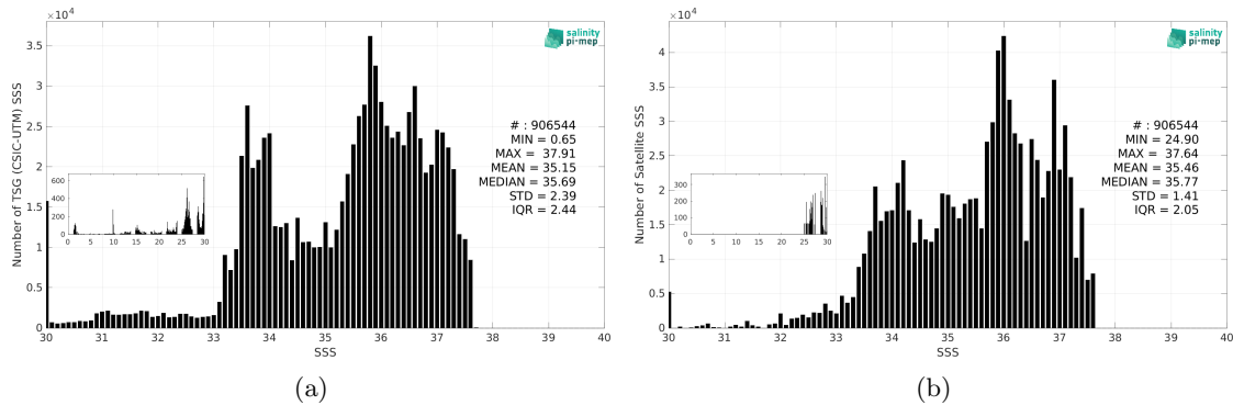
Figure 3: Histograms of SSS from TSG (CSIC-UTM) (a) and SMAP SSS L4 OI v3 - Daily (ESR) (b) considering all match-up pairs per bins of 0.1 over the South Atlantic Ocean Pi-MEP region and for the full satellite product period.
