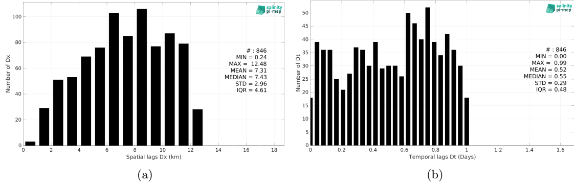
Figure 6: Histograms of the spatial (a) and temporal (b) lags between the location/time of the Saildrone measurement and the date of the corresponding SMAP SSS L4 OI v3 - Daily (ESR) SSS pixel.
