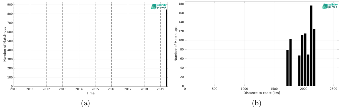
Figure 2: Number of match-ups between Saildrone and SMAP SSS L4 OI v3 - Daily (ESR) SSS as a function of time (a) and as function of the distance to coast (b) over the South Atlantic Ocean Pi-MEP region and for the full satellite product period.
