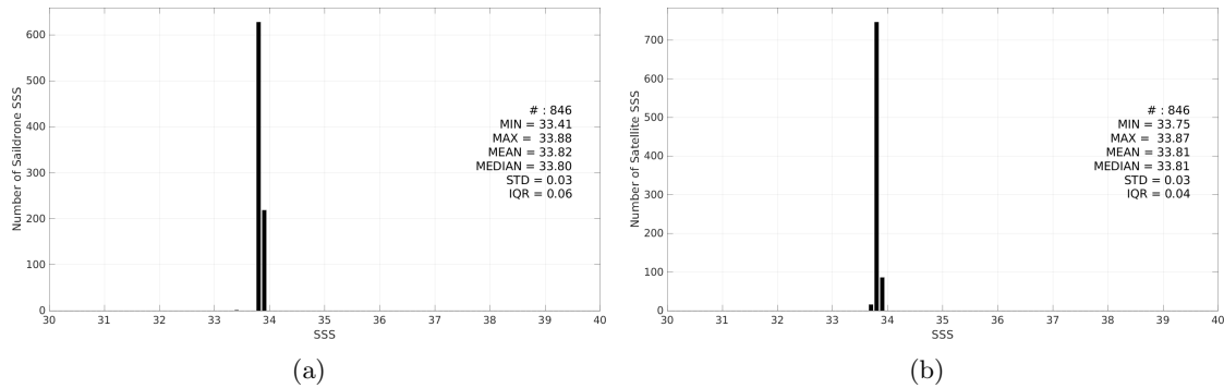
Figure 3: Histograms of SSS from Saildrone (a) and SMAP SSS L4 OI v3 - Daily (ESR) (b) considering all match-up pairs per bins of 0.1 over the South Atlantic Ocean Pi-MEP region and for the full satellite product period.
