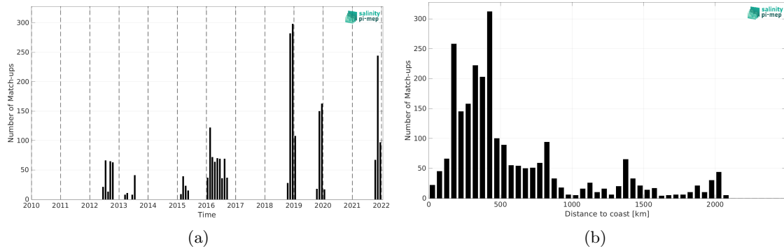
Figure 2: Number of match-ups between Marine mammals and SMAP SSS L4 OI v3 - Daily (ESR) SSS as a function of time (a) and as function of the distance to coast (b) over the South Atlantic Ocean Pi-MEP region and for the full satellite product period.
