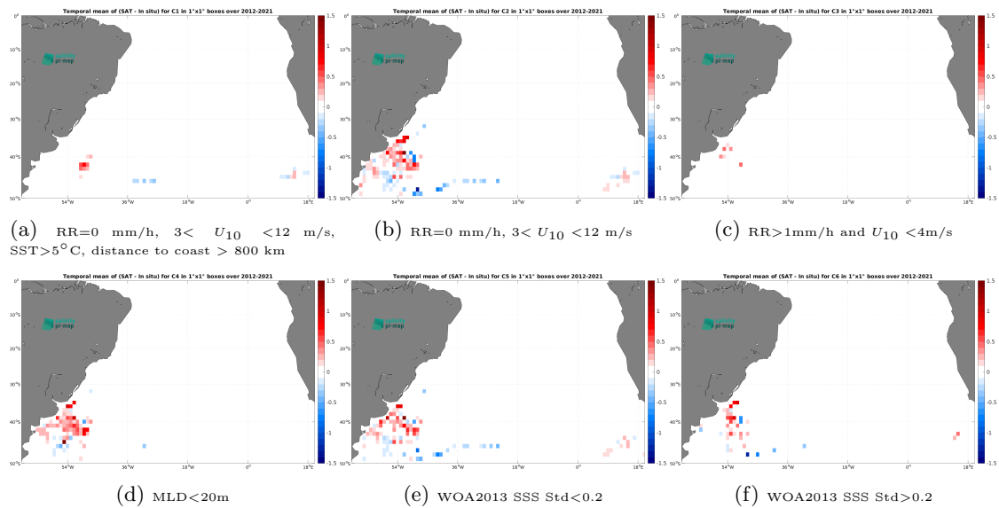
Figure 14: Temporal mean gridded over spatial boxes of size 1^\circ \times 1^\circ of \Delta SSS (SMAP SSS L4 OI v3 - Daily (ESR) - Marine mammals) for 6 different subdatasets corresponding to:RR=0 mm/h, 3 < U_{10} < 12 m/s, SST >5^\circ C, distance to coast > 800 km (a), RR=0 mm/h, 3 < U_{10} < 12 m/s (b), RR >1 mm/h and U_{10} < 4 m/s (c),MLD <20 m (d),WOA2013 SSS Std <0.2 (e),WOA2013 SSS Std >0.2 (f).
