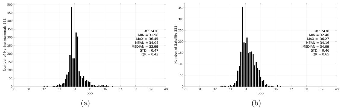
Figure 3: Histograms of SSS from Marine mammals (a) and SMAP SSS L4 OI v3 - Daily (ESR) (b) considering all match-up pairs per bins of 0.1 over the South Atlantic Ocean Pi-MEP region and for the full satellite product period.
