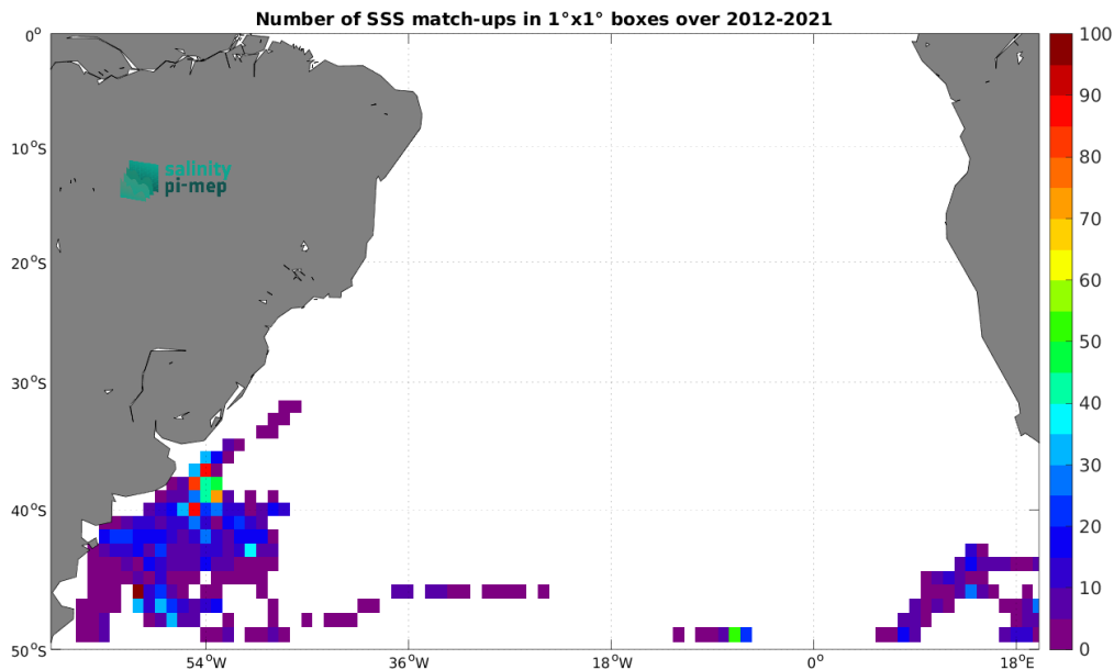
Figure 5: Number of SSS match-ups between Marine mammals SSS and the SMAP SSS L4 OI v3 - Daily (ESR) SSS product for the South Atlantic Ocean Pi-MEP region over 1^\circ \times 1^\circ boxes and for the full satellite product period.
