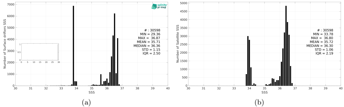
Figure 3: Histograms of SSS from Surface drifters (a) and SMAP SSS L4 OI v3 - Daily (ESR) (b) considering all match-up pairs per bins of 0.1 over the South Atlantic Ocean Pi-MEP region and for the full satellite product period.
