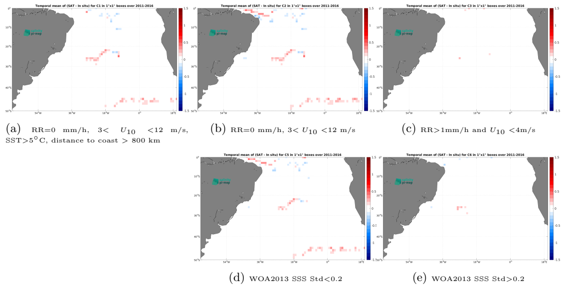
Figure 13: Temporal mean gridded over spatial boxes of size 1^\circ \times 1^\circ of \Delta SSS (SMAP SSS L4 OI v3 - Daily (ESR) - Surface drifters) for 5 different subdatasets corresponding to:RR=0 mm/h, 3 < U_{10} < 12 m/s, SST >5^\circ\text{C} , distance to coast > 800 km (a), RR=0 mm/h, 3 < U_{10} < 12 m/s (b), RR >1 mm/h and U_{10} < 4 m/s (c), WOA2013 SSS Std <0.2 (d), WOA2013 SSS Std >0.2 (e).
