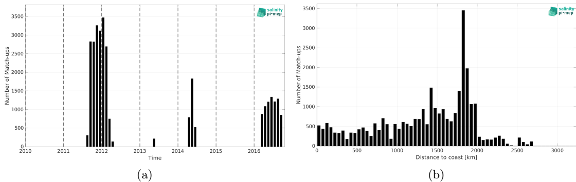
Figure 2: Number of match-ups between Surface drifters and SMAP SSS L4 OI v3 - Daily (ESR) SSS as a function of time (a) and as function of the distance to coast (b) over the South Atlantic Ocean Pi-MEP region and for the full satellite product period.
