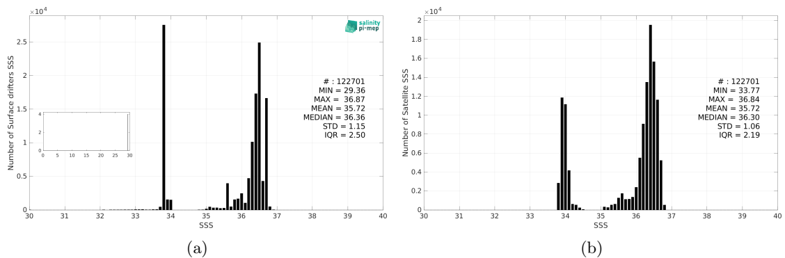
Figure 3: Histograms of SSS from Surface drifters (a) and SMAP SSS L4 OI v3 - Daily (ESR) (b) considering all match-up pairs per bins of 0.1 over the South Atlantic Ocean Pi-MEP region and for the full satellite product period.
