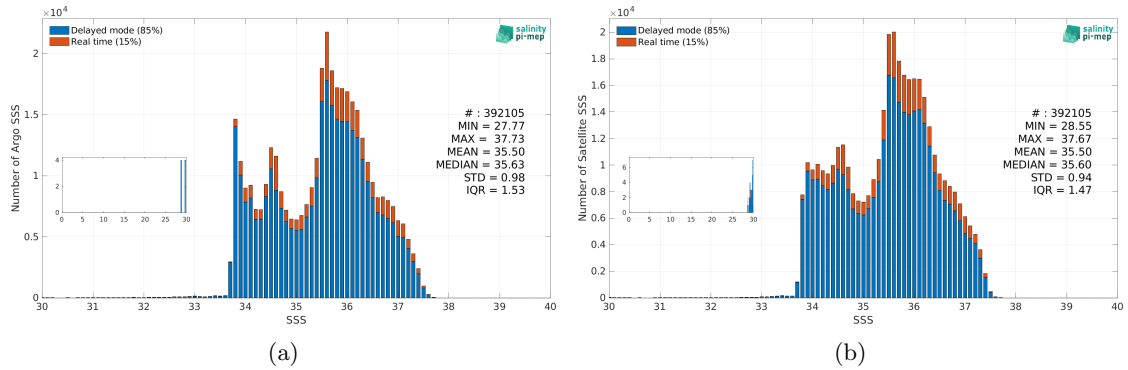
Figure 3: Histograms of SSS from Argo (a) and SMAP SSS L4 OI v3 - Daily (ESR) (b) considering all match-up pairs per bins of 0.1 over the South Atlantic Ocean Pi-MEP region and for the full satellite product period.
