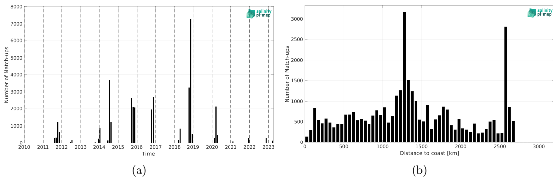
Figure 1: Number of match-ups between TSG (SAMOS) and SMAP SSS L4 OI v2 - 7 Days (ESR) SSS as a function of time (a) and as function of the distance to coast (b) over the South Atlantic Ocean Pi-MEP region and for the full satellite product period.
