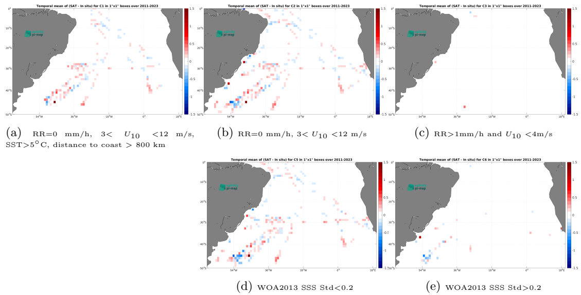
Figure 12: Temporal mean gridded over spatial boxes of size 1^\circ \times 1^\circ of \Delta SSS (SMAP SSS L4 OI v2 - 7 Days (ESR) - TSG (SAMOS)) for 5 different subdatasets corresponding to: RR=0 mm/h, 3 < U_{10} < 12 m/s, SST >5^\circ\text{C} , distance to coast > 800 km (a), RR=0 mm/h, 3 < U_{10} < 12 m/s (b), RR >1 mm/h and U_{10} < 4 m/s (c), WOA2013 SSS Std <0.2 (d), WOA2013 SSS Std >0.2 (e).
