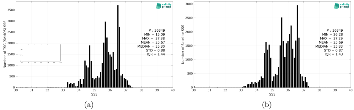
Figure 2: Histograms of SSS from TSG (SAMOS) (a) and SMAP SSS L4 OI v2 - 7 Days (ESR) (b) considering all match-up pairs per bins of 0.1 over the South Atlantic Ocean Pi-MEP region and for the full satellite product period.
