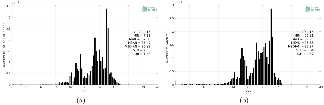
Figure 2: Histograms of SSS from TSG (SAMOS) (a) and SMAP SSS L4 OI v2 - 7 Days (ESR) (b) considering all match-up pairs per bins of 0.1 over the South Atlantic Ocean Pi-MEP region and for the full satellite product period.
