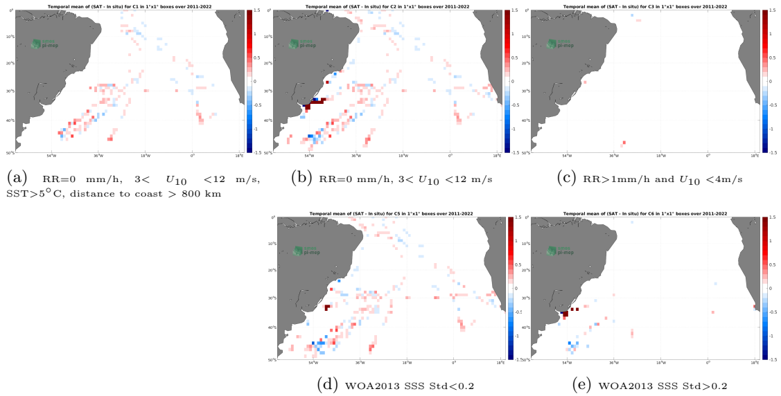
Figure 12: Temporal mean gridded over spatial boxes of size 1^\circ \times 1^\circ of \Delta SSS (SMAP SSS L4 OI v2 - 7 Days (ESR) - TSG (SAMOS)) for 5 different subdatasets corresponding to:RR=0 mm/h, 3 < U_{10} < 12 m/s, SST >5^\circ\text{C} , distance to coast > 800 km (a), RR=0 mm/h, 3 < U_{10} < 12 m/s (b), RR >1 mm/h and U_{10} < 4 m/s (c), WOA2013 SSS Std <0.2 (d), WOA2013 SSS Std >0.2 (e).
