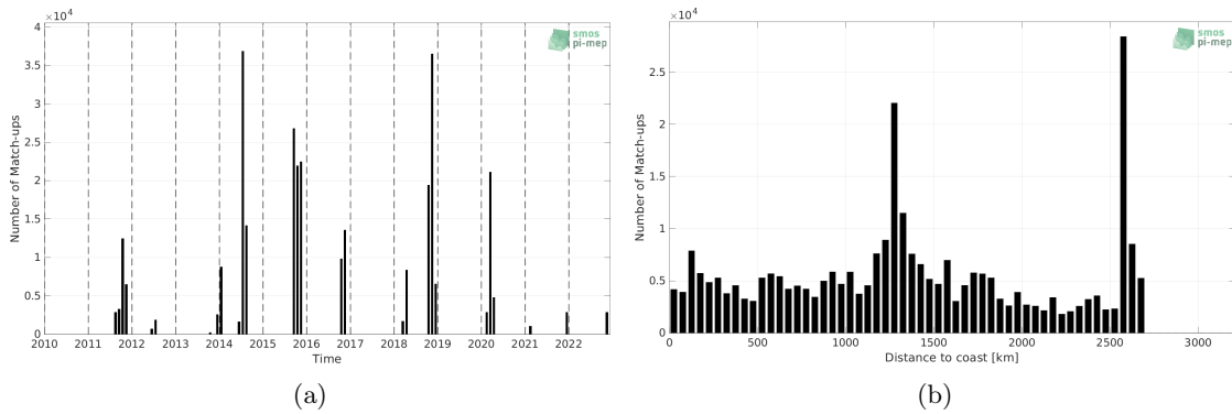
Figure 1: Number of match-ups between TSG (SAMOS) and SMAP SSS L4 OI v2 - 7 Days (ESR) SSS as a function of time (a) and as function of the distance to coast (b) over the South Atlantic Ocean Pi-MEP region and for the full satellite product period.
