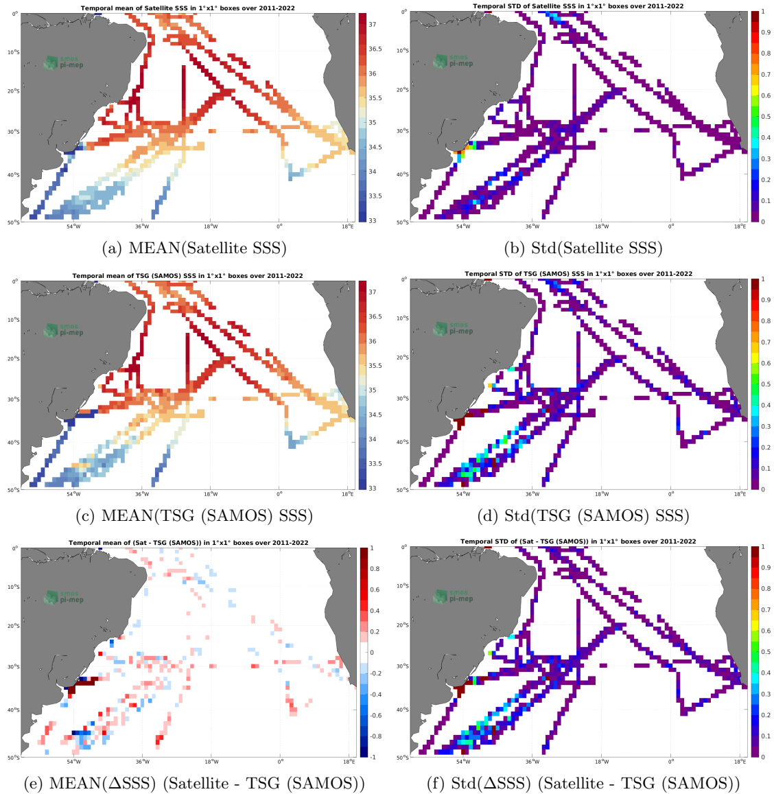
Figure 6: Temporal mean (left) and Std (right) of SSS from SMAP SSS L4 OI v2 - 7 Days (ESR) (top), TSG (SAMOS) (middle), and of \Delta SSS (Satellite - TSG (SAMOS)). Only match-up pairs are used to generate these maps.
