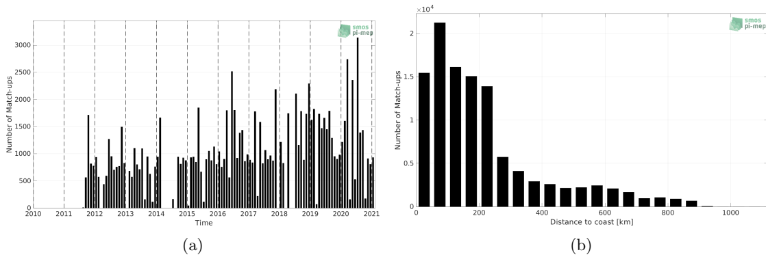
Figure 1: Number of match-ups between TSG (LEGOS-DM) and SMAP SSS L4 OI v2 - 7 Days (ESR) SSS as a function of time (a) and as function of the distance to coast (b) over the South Atlantic Ocean Pi-MEP region and for the full satellite product period.
