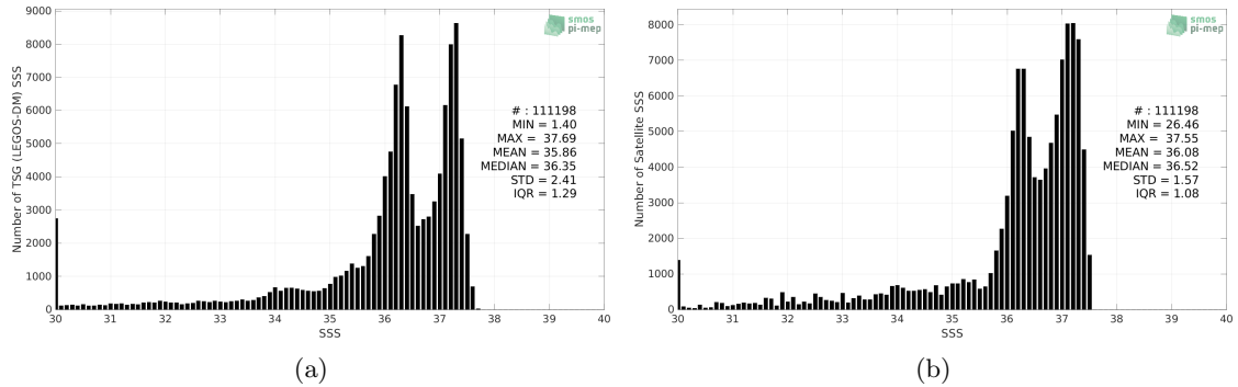
Figure 2: Histograms of SSS from TSG (LEGOS-DM) (a) and SMAP SSS L4 OI v2 - 7 Days (ESR) (b) considering all match-up pairs per bins of 0.1 over the South Atlantic Ocean Pi-MEP region and for the full satellite product period.
