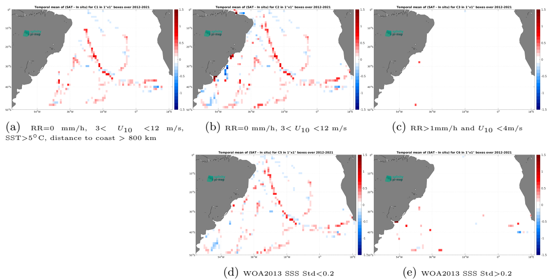
Figure 12: Temporal mean gridded over spatial boxes of size 1^\circ \times 1^\circ of \Delta\text{SSS} (SMAP SSS L4 OI v2 - 7 Days (ESR) - TSG (GOSUD-Sailing-ship)) for 5 different subdatasets corresponding to:RR=0 mm/h, 3 < U_{10} < 12 m/s, SST >5^\circ\text{C} , distance to coast > 800 km (a), RR=0 mm/h, 3 < U_{10} < 12 m/s (b), RR >1 mm/h and U_{10} < 4 m/s (c), WOA2013 SSS Std <0.2 (d), WOA2013 SSS Std >0.2 (e).
