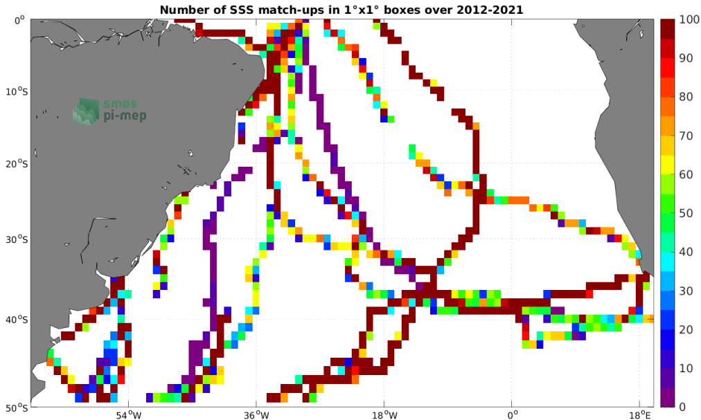
Figure 4: Number of SSS match-ups between TSG (GOSUD-Sailing-ship) SSS and the SMAP SSS L4 OI v2 - 7 Days (ESR) SSS product for the South Atlantic Ocean Pi-MEP region over 1^\circ \times 1^\circ boxes and for the full satellite product period.
