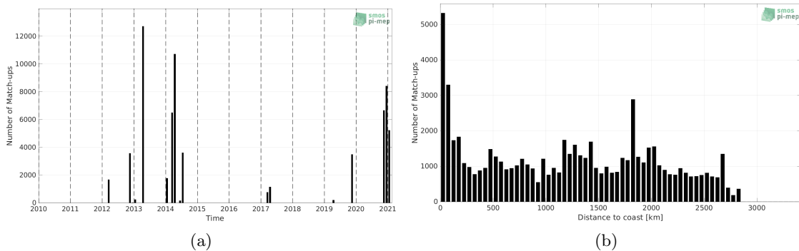
Figure 1: Number of match-ups between TSG (GOSUD-Sailing-ship) and SMAP SSS L4 OI v2 - 7 Days (ESR) SSS as a function of time (a) and as function of the distance to coast (b) over the South Atlantic Ocean Pi-MEP region and for the full satellite product period.
