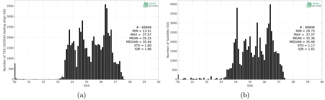
Figure 2: Histograms of SSS from TSG (GOSUD-Sailing-ship) (a) and SMAP SSS L4 OI v2 - 7 Days (ESR) (b) considering all match-up pairs per bins of 0.1 over the South Atlantic Ocean Pi-MEP region and for the full satellite product period.
