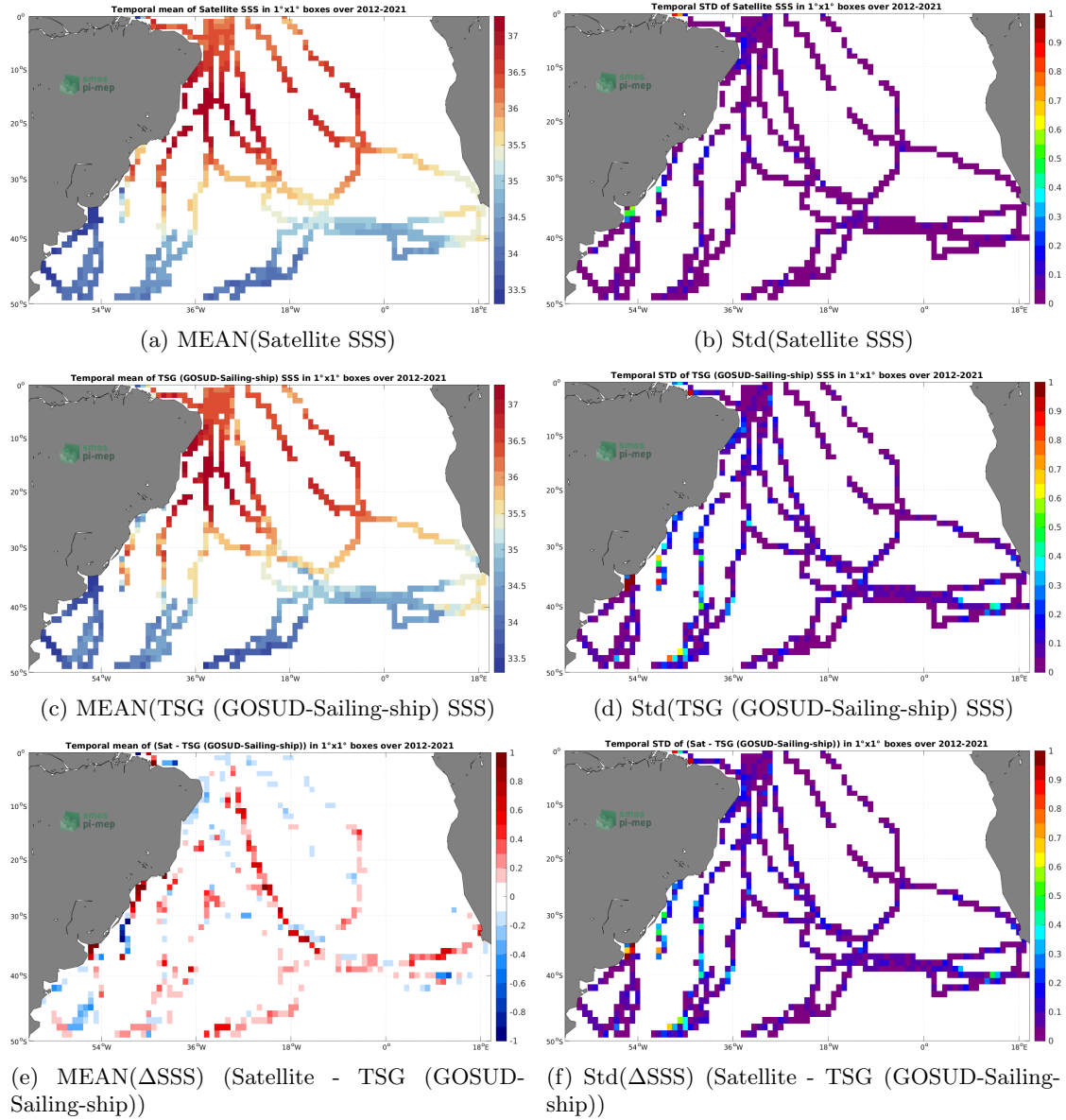
Figure 6: Temporal mean (left) and Std (right) of SSS from SMAP SSS L4 OI v2 - 7 Days (ESR) (top), TSG (GOSUD-Sailing-ship) (middle), and of \Delta SSS (Satellite - TSG (GOSUD-Sailing-ship)). Only match-up pairs are used to generate these maps.
