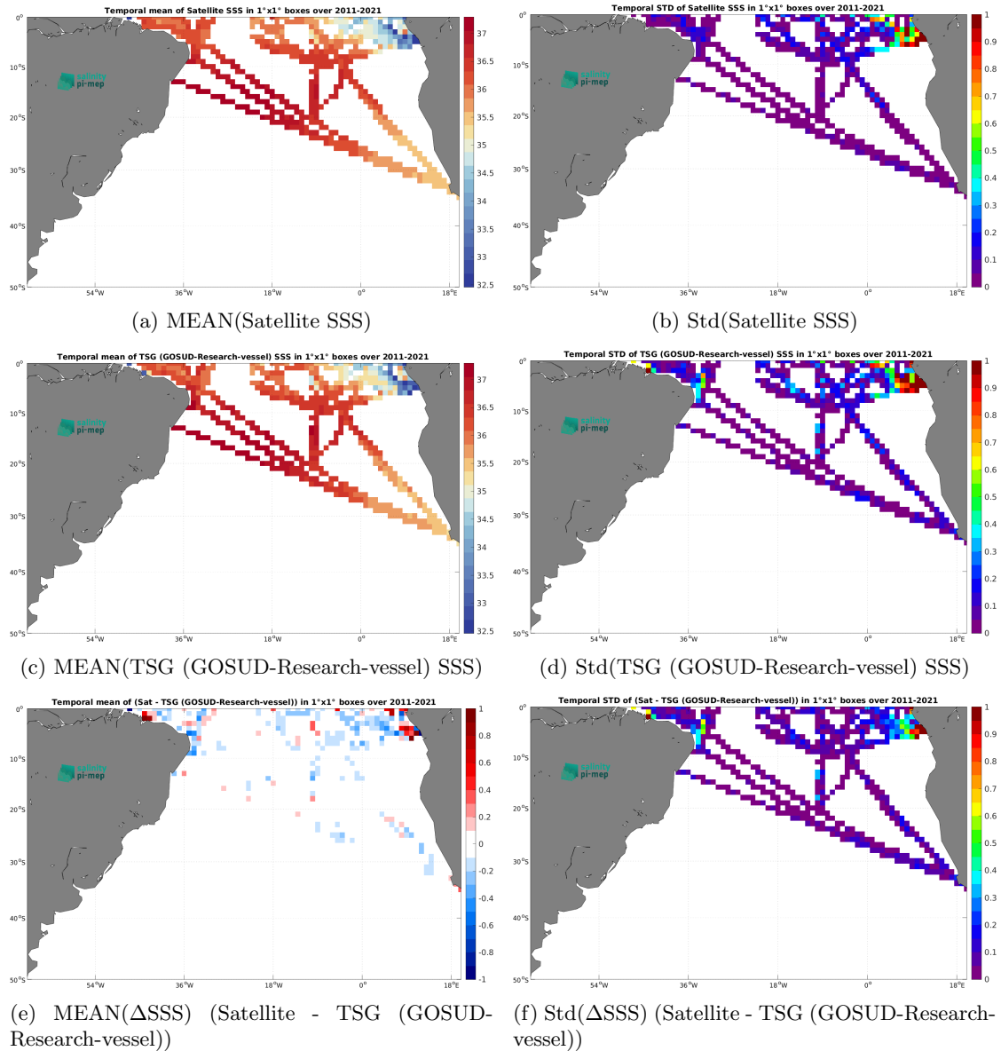
Figure 6: Temporal mean (left) and Std (right) of SSS from SMAP SSS L4 OI v2 - 7 Days (ESR) (top), TSG (GOSUD-Research-vessel) (middle), and of \Delta SSS (Satellite - TSG (GOSUD-Research-vessel)). Only match-up pairs are used to generate these maps.
