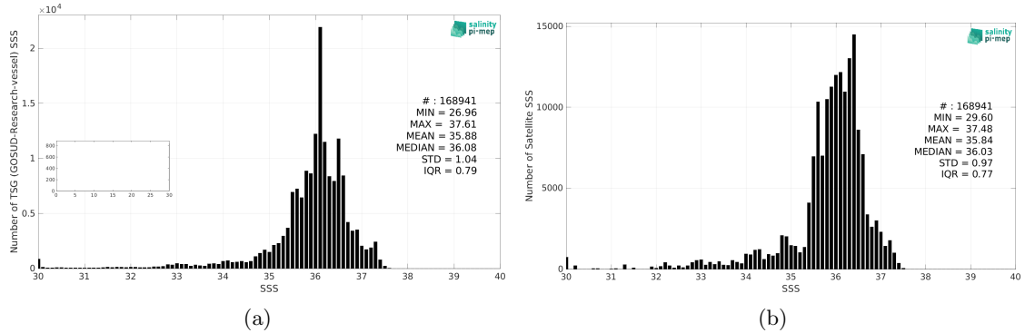
Figure 2: Histograms of SSS from TSG (GOSUD-Research-vessel) (a) and SMAP SSS L4 OI v2 - 7 Days (ESR) (b) considering all match-up pairs per bins of 0.1 over the South Atlantic Ocean Pi-MEP region and for the full satellite product period.
