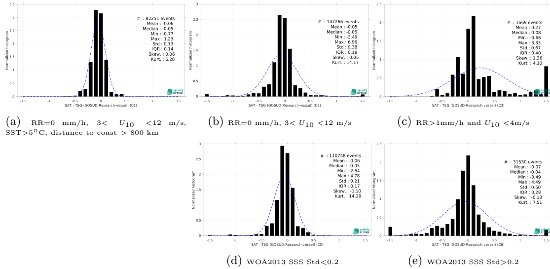
Figure 13: Normalized histogram of \Delta SSS (SMAP SSS L4 OI v2 - 7 Days (ESR) - TSG (GOSUD-Research-vessel)) for 5 different subdatasets corresponding to: RR=0 mm/h, 3 < U_{10} < 12 m/s, SST>5°C, distance to coast > 800 km (a), RR=0 mm/h, 3 < U_{10} < 12 m/s (b), RR>1mm/h and U_{10} < 4 m/s (c), WOA2013 SSS Std<0.2 (d), WOA2013 SSS Std>0.2 (e).
