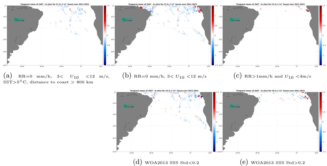
Figure 12: Temporal mean gridded over spatial boxes of size 1^\circ \times 1^\circ of \Delta SSS (SMAP SSS L4 OI v2 - 7 Days (ESR) - TSG (GOSUD-Research-vessel)) for 5 different subdatasets corresponding to:RR=0 mm/h, 3 < U_{10} < 12 m/s, SST >5^\circ C, distance to coast > 800 km (a), RR=0 mm/h, 3 < U_{10} < 12 m/s (b), RR >1 mm/h and U_{10} < 4 m/s (c), WOA2013 SSS Std <0.2 (d), WOA2013 SSS Std >0.2 (e).
