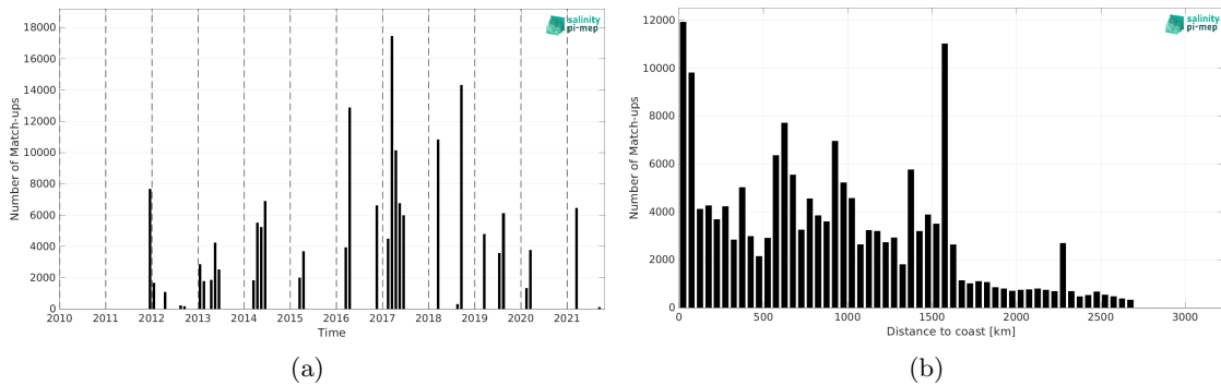
Figure 1: Number of match-ups between TSG (GOSUD-Research-vessel) and SMAP SSS L4 OI v2 - 7 Days (ESR) SSS as a function of time (a) and as function of the distance to coast (b) over the South Atlantic Ocean Pi-MEP region and for the full satellite product period.
