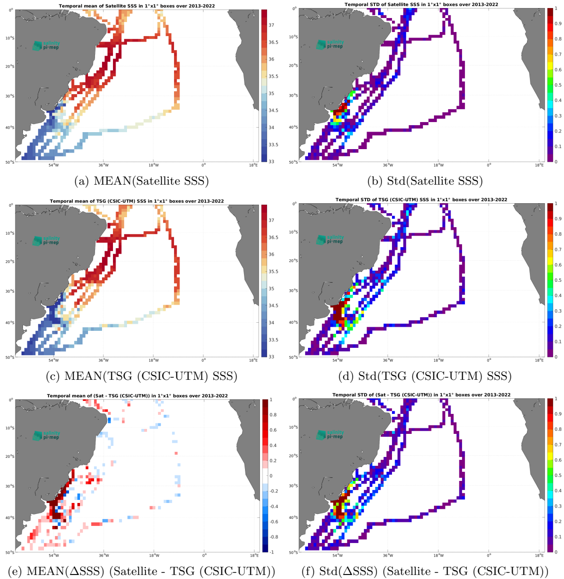
Figure 6: Temporal mean (left) and Std (right) of SSS from SMAP SSS L4 OI v2 - 7 Days (ESR) (top), TSG (CSIC-UTM) (middle), and of \Delta SSS (Satellite - TSG (CSIC-UTM)). Only match-up pairs are used to generate these maps.
