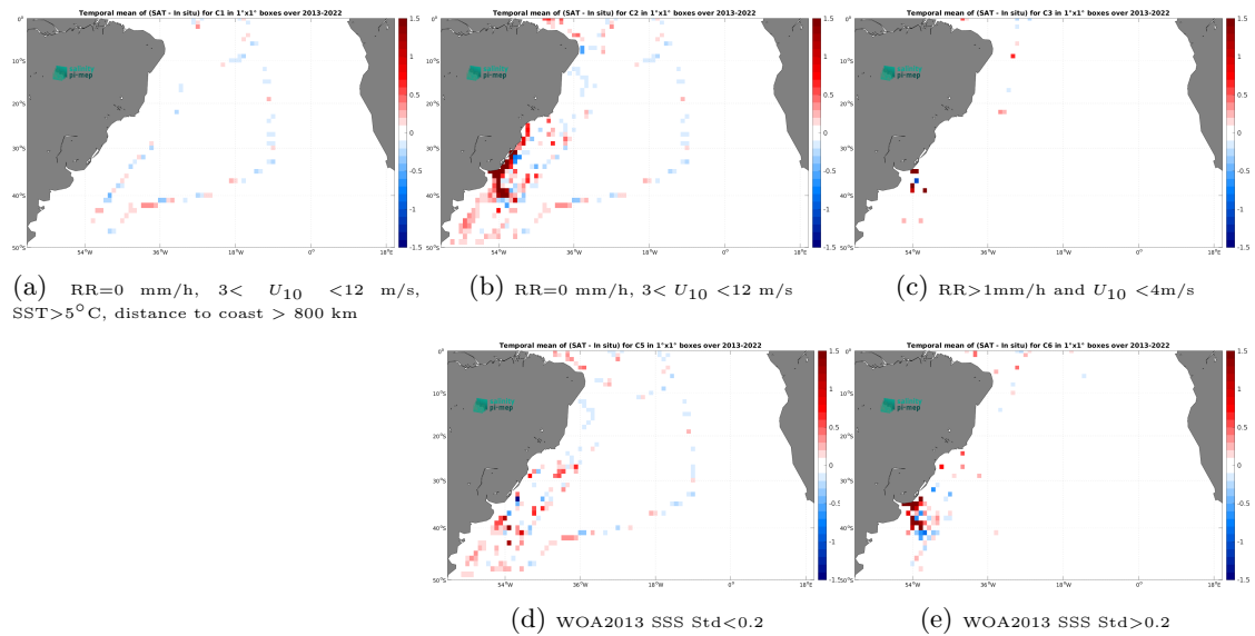
Figure 12: Temporal mean gridded over spatial boxes of size 1^\circ \times 1^\circ of \Delta\text{SSS} (SMAP SSS L4 OI v2 - 7 Days (ESR) - TSG (CSIC-UTM)) for 5 different subdatasets corresponding to:RR=0 mm/h, 3 < U_{10} < 12 m/s, SST >5^\circ\text{C} , distance to coast > 800 km (a), RR=0 mm/h, 3 < U_{10} < 12 m/s (b), RR >1 mm/h and U_{10} < 4 m/s (c), WOA2013 SSS Std <0.2 (d), WOA2013 SSS Std >0.2 (e).
