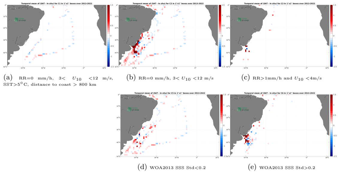
Figure 12: Temporal mean gridded over spatial boxes of size 1^\circ \times 1^\circ of \Delta SSS (SMAP SSS L4 OI v2 - 7 Days (ESR) - TSG (CSIC-UTM)) for 5 different subdatasets corresponding to:RR=0 mm/h, 3 < U_{10} < 12 m/s, SST >5^\circ\text{C} , distance to coast > 800 km (a), RR=0 mm/h, 3 < U_{10} < 12 m/s (b), RR >1 mm/h and U_{10} < 4 m/s (c), WOA2013 SSS Std <0.2 (d), WOA2013 SSS Std >0.2 (e).
