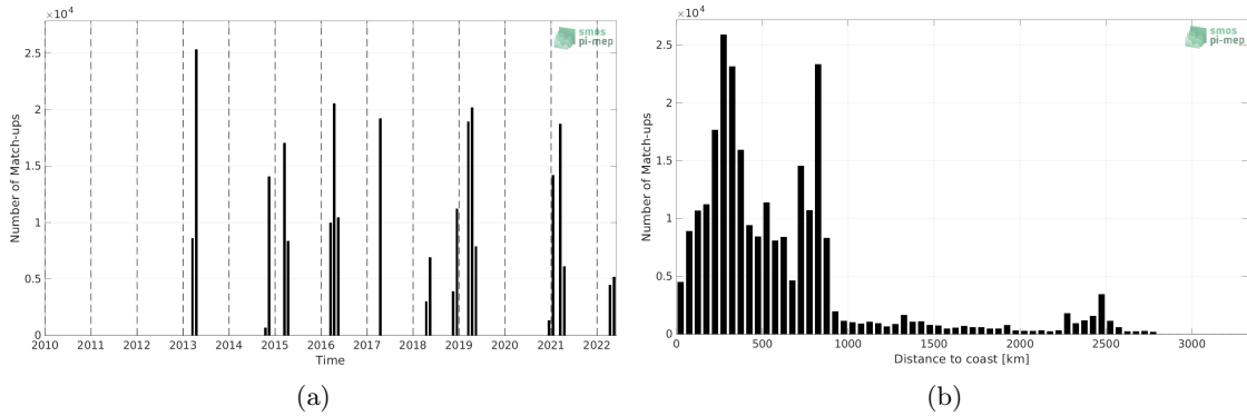
Figure 1: Number of match-ups between TSG (CSIC-UTM) and SMAP SSS L4 OI v2 - 7 Days (ESR) SSS as a function of time (a) and as function of the distance to coast (b) over the South Atlantic Ocean Pi-MEP region and for the full satellite product period.
