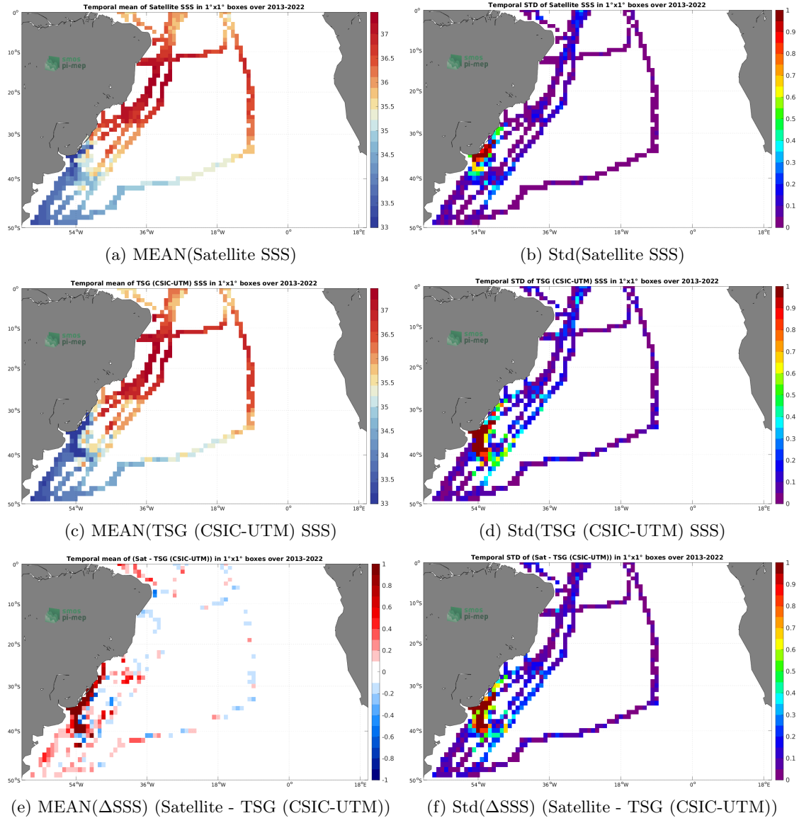
Figure 6: Temporal mean (left) and Std (right) of SSS from SMAP SSS L4 OI v2 - 7 Days (ESR) (top), TSG (CSIC-UTM) (middle), and of \Delta SSS (Satellite - TSG (CSIC-UTM)). Only match-up pairs are used to generate these maps.
