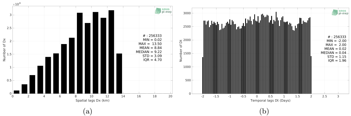
Figure 5: Histograms of the spatial (a) and temporal (b) lags between the location/time of the TSG (CSIC-UTM) measurement and the date of the corresponding SMAP SSS L4 OI v2 - 7 Days (ESR) SSS pixel.
