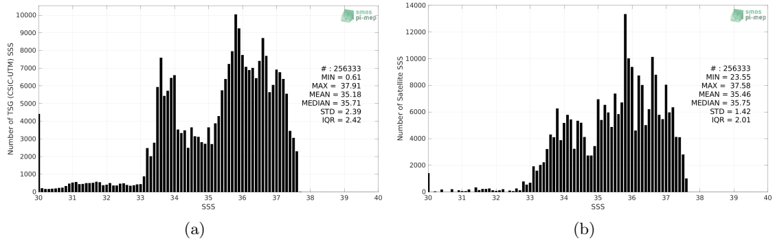
Figure 2: Histograms of SSS from TSG (CSIC-UTM) (a) and SMAP SSS L4 OI v2 - 7 Days (ESR) (b) considering all match-up pairs per bins of 0.1 over the South Atlantic Ocean Pi-MEP region and for the full satellite product period.
