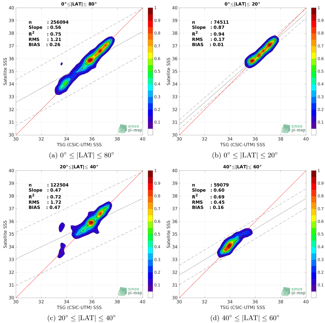
Figure 9: Contour maps of the concentration of SMAP SSS L4 OI v2 - 7 Days (ESR) SSS ( y -axis) versus TSG (CSIC-UTM) SSS ( x -axis) at match-up pairs for different latitude bands. For each plot, the red line shows x=y . The black thin and dashed lines indicate a linear fit through the data cloud and the \pm 95\% confidence levels, respectively. The number match-up pairs n , the slope and R^2 coefficient of the linear fit, the root mean square (RMS) and the mean bias between satellite and in situ data are indicated for each latitude band in each plots.
