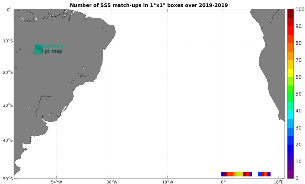
Figure 4: Number of SSS match-ups between Saildrone SSS and the SMAP SSS L4 OI v2 - 7 Days (ESR) SSS product for the South Atlantic Ocean Pi-MEP region over 1^\circ \times 1^\circ boxes and for the full satellite product period.
