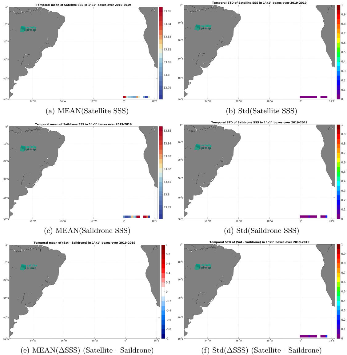
Figure 6: Temporal mean (left) and Std (right) of SSS from SMAP SSS L4 OI v2 - 7 Days (ESR) (top), Saildrone (middle), and of \Delta SSS (Satellite - Saildrone). Only match-up pairs are used to generate these maps.
