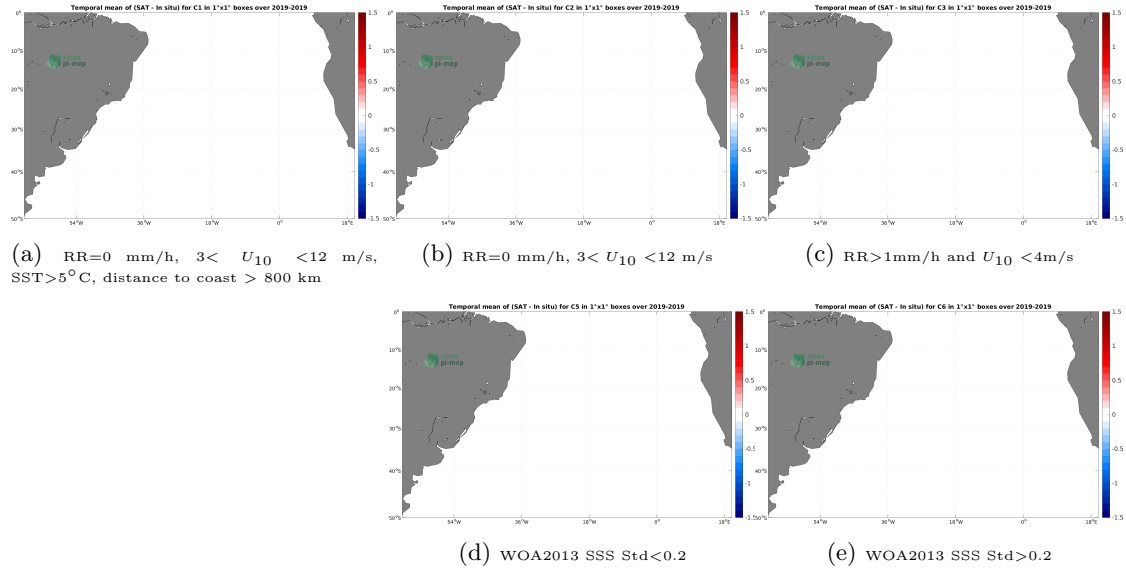
Figure 12: Temporal mean gridded over spatial boxes of size 1^{\circ}\times 1^{\circ} of \Delta\text{SSS} (SMAP SSS L4 OI v2 - 7 Days (ESR) - Sairdrone) for 5 different subdatasets corresponding to:RR=0 mm/h, 3 < U_{10} < 12 m/s, SST >5^{\circ}\text{C} , distance to coast > 800 km (a), RR=0 mm/h, 3 < U_{10} < 12 m/s (b), RR >1 mm/h and U_{10} < 4 m/s (c), WOA2013 SSS Std <0.2 (d), WOA2013 SSS Std >0.2 (e).
