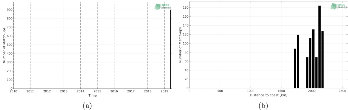
Figure 1: Number of match-ups between Saildrone and SMAP SSS L4 OI v2 - 7 Days (ESR) SSS as a function of time (a) and as function of the distance to coast (b) over the South Atlantic Ocean Pi-MEP region and for the full satellite product period.
