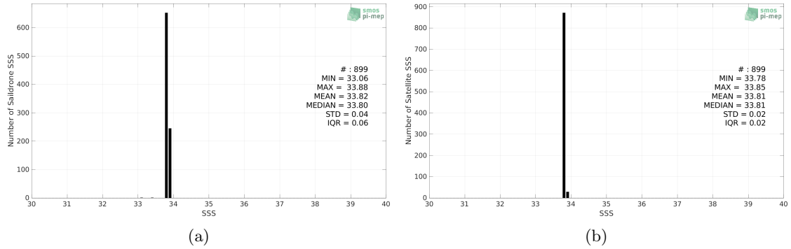
Figure 2: Histograms of SSS from Saildrone (a) and SMAP SSS L4 OI v2 - 7 Days (ESR) (b) considering all match-up pairs per bins of 0.1 over the South Atlantic Ocean Pi-MEP region and for the full satellite product period.
