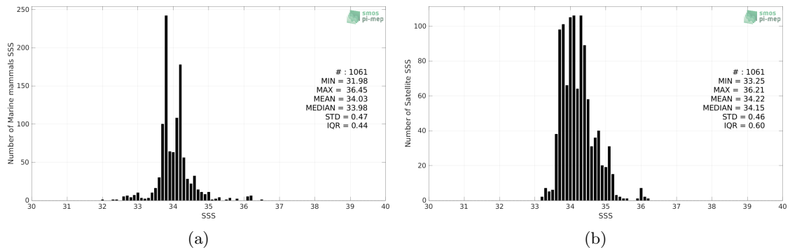
Figure 2: Histograms of SSS from Marine mammals (a) and SMAP SSS L4 OI v2 - 7 Days (ESR) (b) considering all match-up pairs per bins of 0.1 over the South Atlantic Ocean Pi-MEP region and for the full satellite product period.
