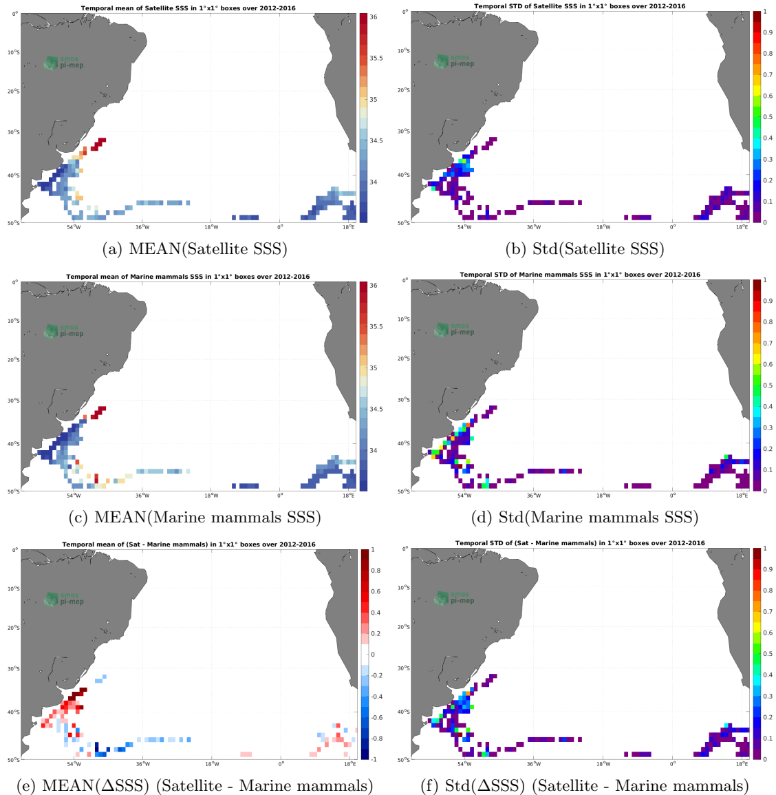
Figure 6: Temporal mean (left) and Std (right) of SSS from SMAP SSS L4 OI v2 - 7 Days (ESR) (top), Marine mammals (middle), and of \Delta SSS (Satellite - Marine mammals). Only match-up pairs are used to generate these maps.
