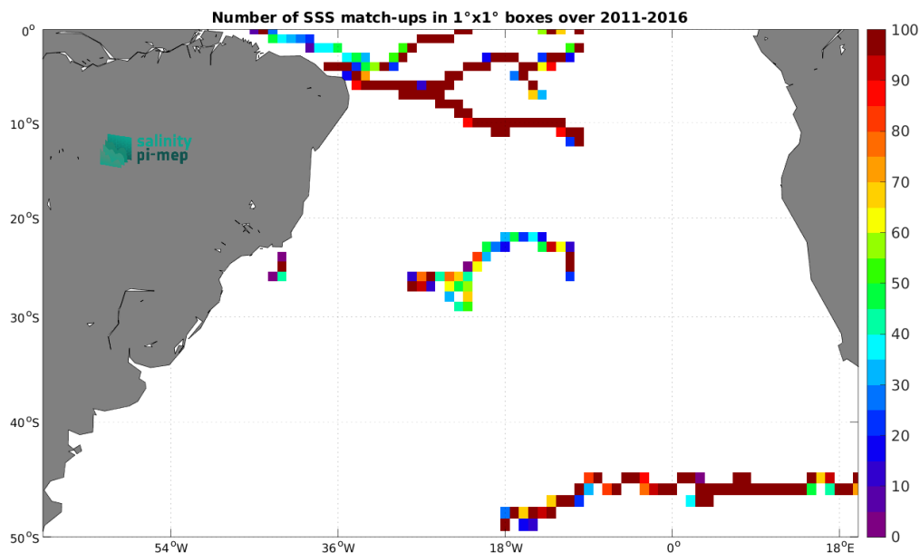
Figure 3: Number of SSS match-ups between Surface drifters SSS and the SMAP SSS L4 OI v2 - 7 Days (ESR) SSS product for the South Atlantic Ocean Pi-MEP region over 1^\circ \times 1^\circ boxes and for the full satellite product period.
