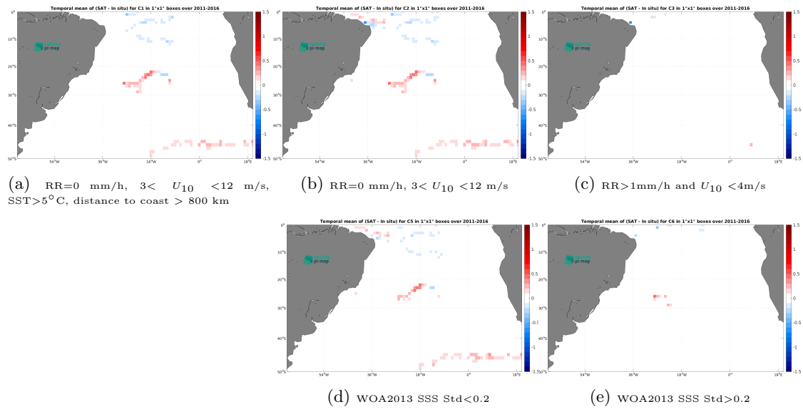
Figure 11: Temporal mean gridded over spatial boxes of size 1^\circ \times 1^\circ of \Delta SSS (SMAP SSS L4 OI v2 - 7 Days (ESR) - Surface drifters) for 5 different subdatasets corresponding to:RR=0 mm/h, 3 < U_{10} < 12 m/s, SST >5^\circ\text{C} , distance to coast > 800 km (a), RR=0 mm/h, 3 < U_{10} < 12 m/s (b), RR >1 mm/h and U_{10} < 4 m/s (c), WOA2013 SSS Std <0.2 (d), WOA2013 SSS Std >0.2 (e).
