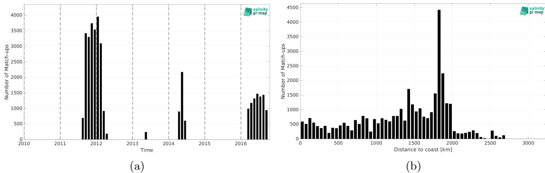
Figure 1: Number of match-ups between Surface drifters and SMAP SSS L4 OI v2 - 7 Days (ESR) SSS as a function of time (a) and as function of the distance to coast (b) over the South Atlantic Ocean Pi-MEP region and for the full satellite product period.
