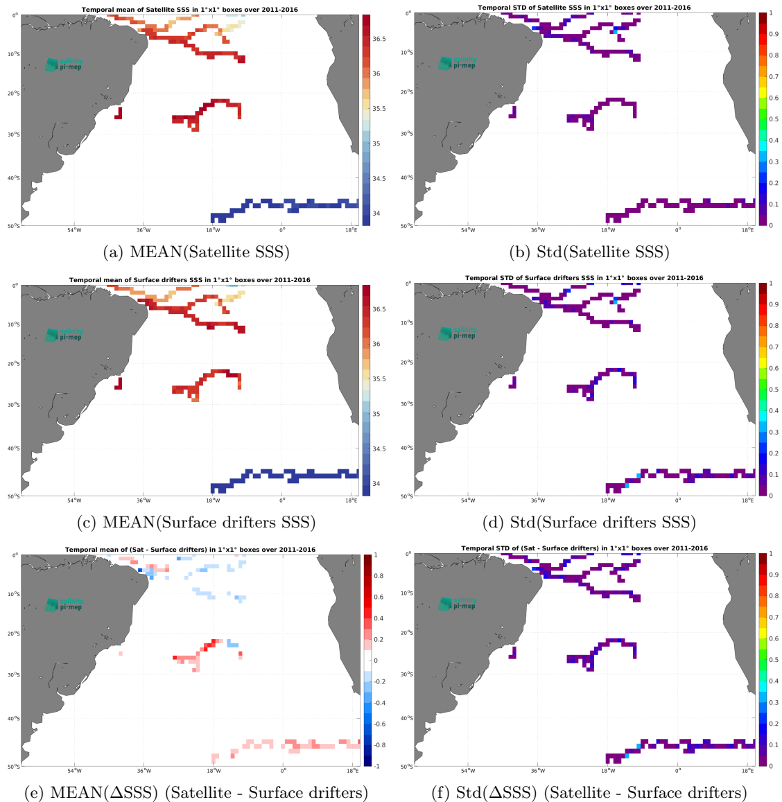
Figure 5: Temporal mean (left) and Std (right) of SSS from SMAP SSS L4 OI v2 - 7 Days (ESR) (top), Surface drifters (middle), and of \Delta SSS (Satellite - Surface drifters). Only match-up pairs are used to generate these maps.
