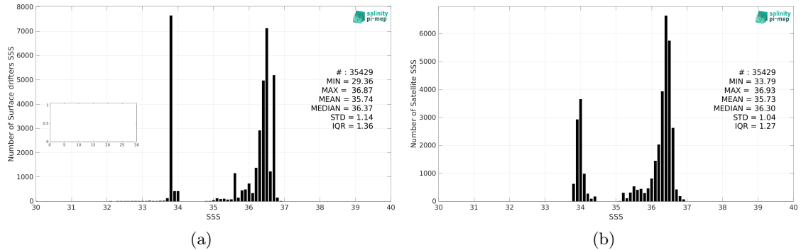
Figure 2: Histograms of SSS from Surface drifters (a) and SMAP SSS L4 OI v2 - 7 Days (ESR) (b) considering all match-up pairs per bins of 0.1 over the South Atlantic Ocean Pi-MEP region and for the full satellite product period.
