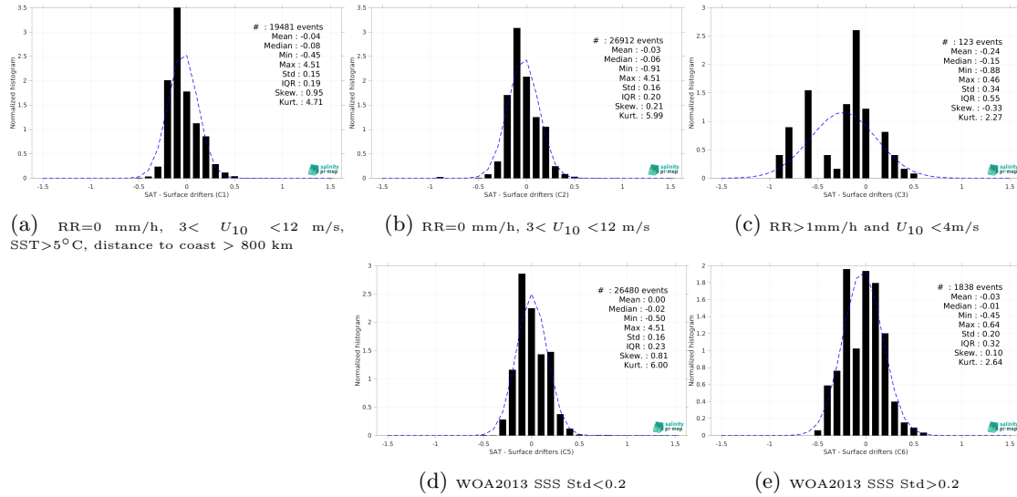
Figure 12: Normalized histogram of \Delta\text{SSS} (SMAP SSS L4 OI v2 - 7 Days (ESR) - Surface drifters) for 5 different subdatasets corresponding to: RR=0 mm/h, 3 < U_{10} < 12 m/s, SST>5°C, distance to coast > 800 km (a), RR=0 mm/h, 3 < U_{10} < 12 m/s (b), RR>1mm/h and U_{10} < 4 m/s (c), WOA2013 SSS Std<0.2 (d), WOA2013 SSS Std>0.2 (e).
