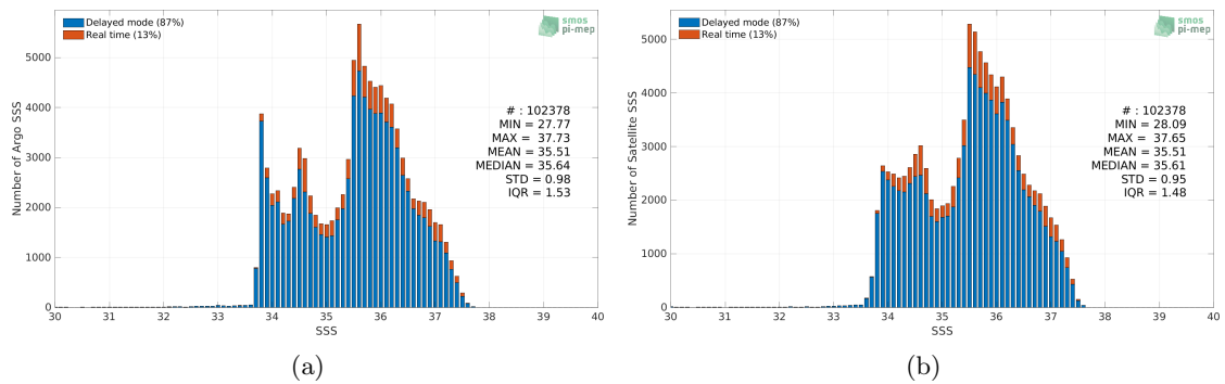
Figure 2: Histograms of SSS from Argo (a) and SMAP SSS L4 OI v2 - 7 Days (ESR) (b) considering all match-up pairs per bins of 0.1 over the South Atlantic Ocean Pi-MEP region and for the full satellite product period.
