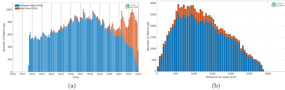
Figure 1: Number of match-ups between Argo and SMAP SSS L4 OI v2 - 7 Days (ESR) SSS as a function of time (a) and as function of the distance to coast (b) over the South Atlantic Ocean Pi-MEP region and for the full satellite product period.
