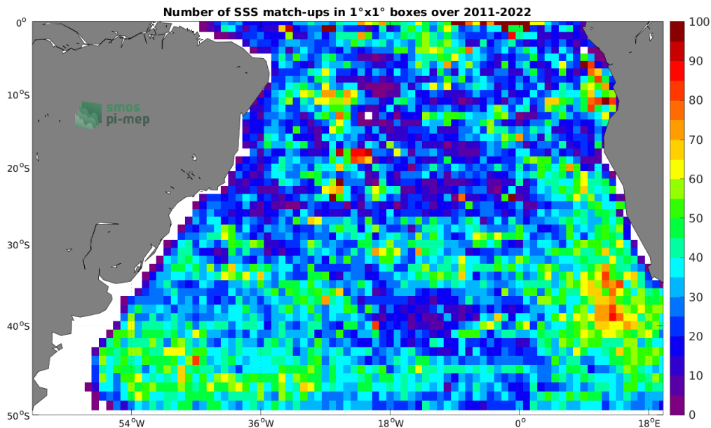
Figure 4: Number of SSS match-ups between Argo SSS and the SMAP SSS L4 OI v2 - 7 Days (ESR) SSS product for the South Atlantic Ocean Pi-MEP region over 1^\circ \times 1^\circ boxes and for the full satellite product period.
