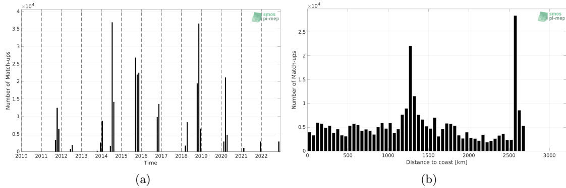
Figure 1: Number of match-ups between TSG (SAMOS) and SMAP SSS L4 OI v2 - Monthly (IPRC) SSS as a function of time (a) and as function of the distance to coast (b) over the South Atlantic Ocean Pi-MEP region and for the full satellite product period.
