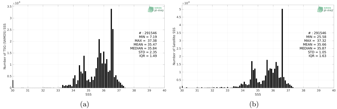
Figure 2: Histograms of SSS from TSG (SAMOS) (a) and SMAP SSS L4 OI v2 - Monthly (IPRC) (b) considering all match-up pairs per bins of 0.1 over the South Atlantic Ocean Pi-MEP region and for the full satellite product period.
