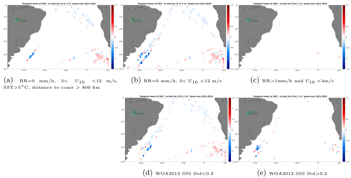
Figure 12: Temporal mean gridded over spatial boxes of size 1^\circ \times 1^\circ of \Delta SSS (SMAP SSS L4 OI v2 - Monthly (IPRC) - TSG (Polarstern)) for 5 different subdatasets corresponding to:RR=0 mm/h, 3 < U_{10} < 12 m/s, SST >5^\circ\text{C} , distance to coast > 800 km (a), RR=0 mm/h, 3 < U_{10} < 12 m/s (b), RR >1 mm/h and U_{10} < 4 m/s (c), WOA2013 SSS Std <0.2 (d), WOA2013 SSS Std >0.2 (e).
