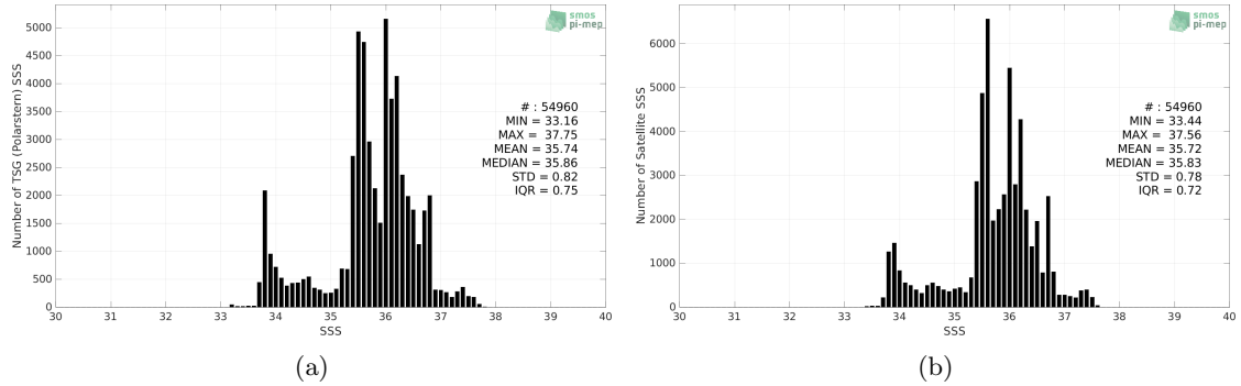
Figure 2: Histograms of SSS from TSG (Polarstern) (a) and SMAP SSS L4 OI v2 - Monthly (IPRC) (b) considering all match-up pairs per bins of 0.1 over the South Atlantic Ocean Pi-MEP region and for the full satellite product period.
