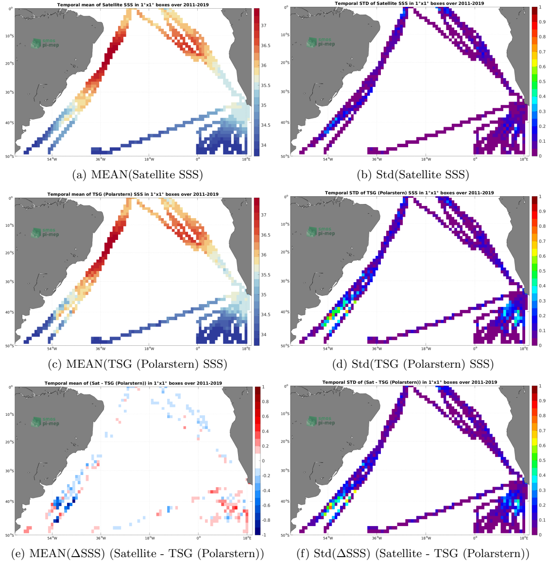
Figure 6: Temporal mean (left) and Std (right) of SSS from SMAP SSS L4 OI v2 - Monthly (IPRC) (top), TSG (Polarstern) (middle), and of \Delta SSS (Satellite - TSG (Polarstern)). Only match-up pairs are used to generate these maps.
