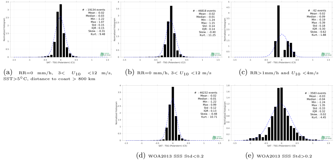
Figure 13: Normalized histogram of \Delta SSS (SMAP SSS L4 OI v2 - Monthly (IPRC) - TSG (Polarstern)) for 5 different subdatasets corresponding to: RR=0 mm/h, 3 < U_{10} < 12 m/s, SST>5°C, distance to coast > 800 km (a), RR=0 mm/h, 3 < U_{10} < 12 m/s (b), RR>1mm/h and U_{10} < 4 m/s (c), WOA2013 SSS Std<0.2 (d), WOA2013 SSS Std>0.2 (e).
