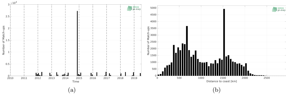
Figure 1: Number of match-ups between TSG (Polarstern) and SMAP SSS L4 OI v2 - Monthly (IPRC) SSS as a function of time (a) and as function of the distance to coast (b) over the South Atlantic Ocean Pi-MEP region and for the full satellite product period.
