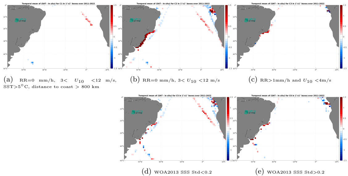
Figure 12: Temporal mean gridded over spatial boxes of size 1^\circ \times 1^\circ of \Delta\text{SSS} (SMAP SSS L4 OI v2 - Monthly (IPRC) - TSG (LEGOS-DM)) for 5 different subdatasets corresponding to:RR=0 mm/h, 3 < U_{10} < 12 m/s, SST >5^\circ\text{C} , distance to coast > 800 km (a), RR=0 mm/h, 3 < U_{10} < 12 m/s (b), RR >1 mm/h and U_{10} < 4 m/s (c), WOA2013 SSS Std <0.2 (d), WOA2013 SSS Std >0.2 (e).
