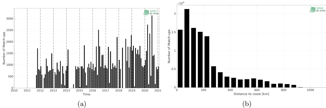
Figure 1: Number of match-ups between TSG (LEGOS-DM) and SMAP SSS L4 OI v2 - Monthly (IPRC) SSS as a function of time (a) and as function of the distance to coast (b) over the South Atlantic Ocean Pi-MEP region and for the full satellite product period.
