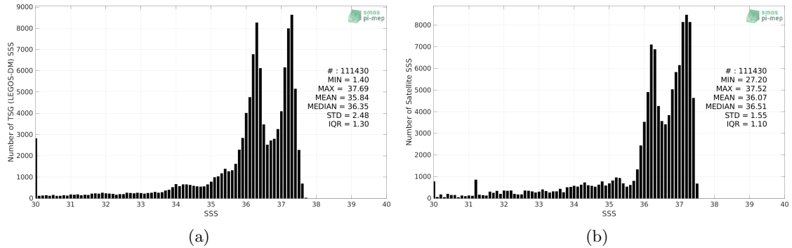
Figure 2: Histograms of SSS from TSG (LEGOS-DM) (a) and SMAP SSS L4 OI v2 - Monthly (IPRC) (b) considering all match-up pairs per bins of 0.1 over the South Atlantic Ocean Pi-MEP region and for the full satellite product period.
