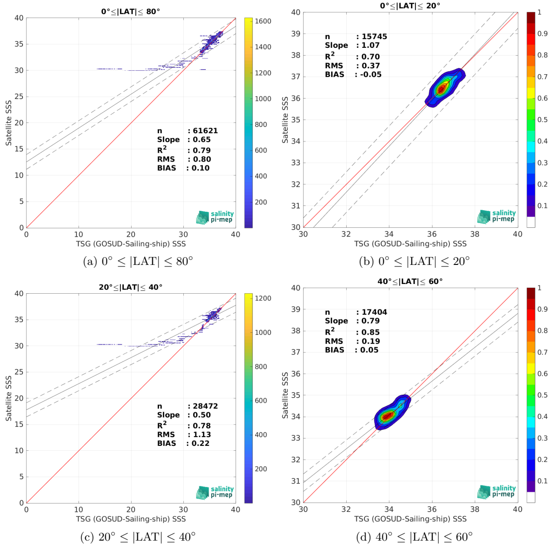
Figure 9: Contour maps of the concentration of SMAP SSS L4 OI v2 - Monthly (IPRC) SSS (y-axis) versus TSG (GOSUD-Sailing-ship) SSS (x-axis) at match-up pairs for different latitude bands. For each plot, the red line shows x=y . The black thin and dashed lines indicate a linear fit through the data cloud and the \pm 95\% confidence levels, respectively. The number match-up pairs n , the slope and R^2 coefficient of the linear fit, the root mean square (RMS) and the mean bias between satellite and in situ data are indicated for each latitude band in each plots.
