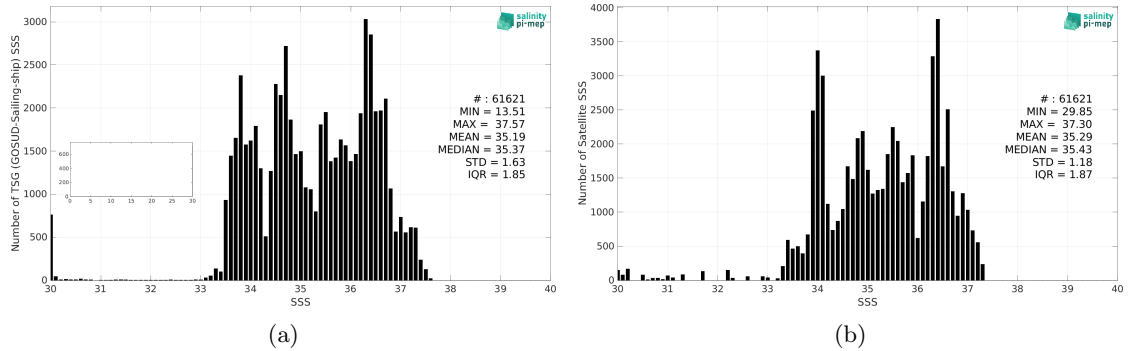
Figure 2: Histograms of SSS from TSG (GOSUD-Sailing-ship) (a) and SMAP SSS L4 OI v2 - Monthly (IPRC) (b) considering all match-up pairs per bins of 0.1 over the South Atlantic Ocean Pi-MEP region and for the full satellite product period.
