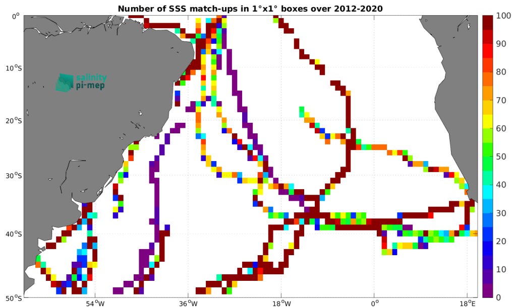
Figure 4: Number of SSS match-ups between TSG (GOSUD-Sailing-ship) SSS and the SMAP SSS L4 OI v2 - Monthly (IPRC) SSS product for the South Atlantic Ocean Pi-MEP region over 1^\circ \times 1^\circ boxes and for the full satellite product period.
