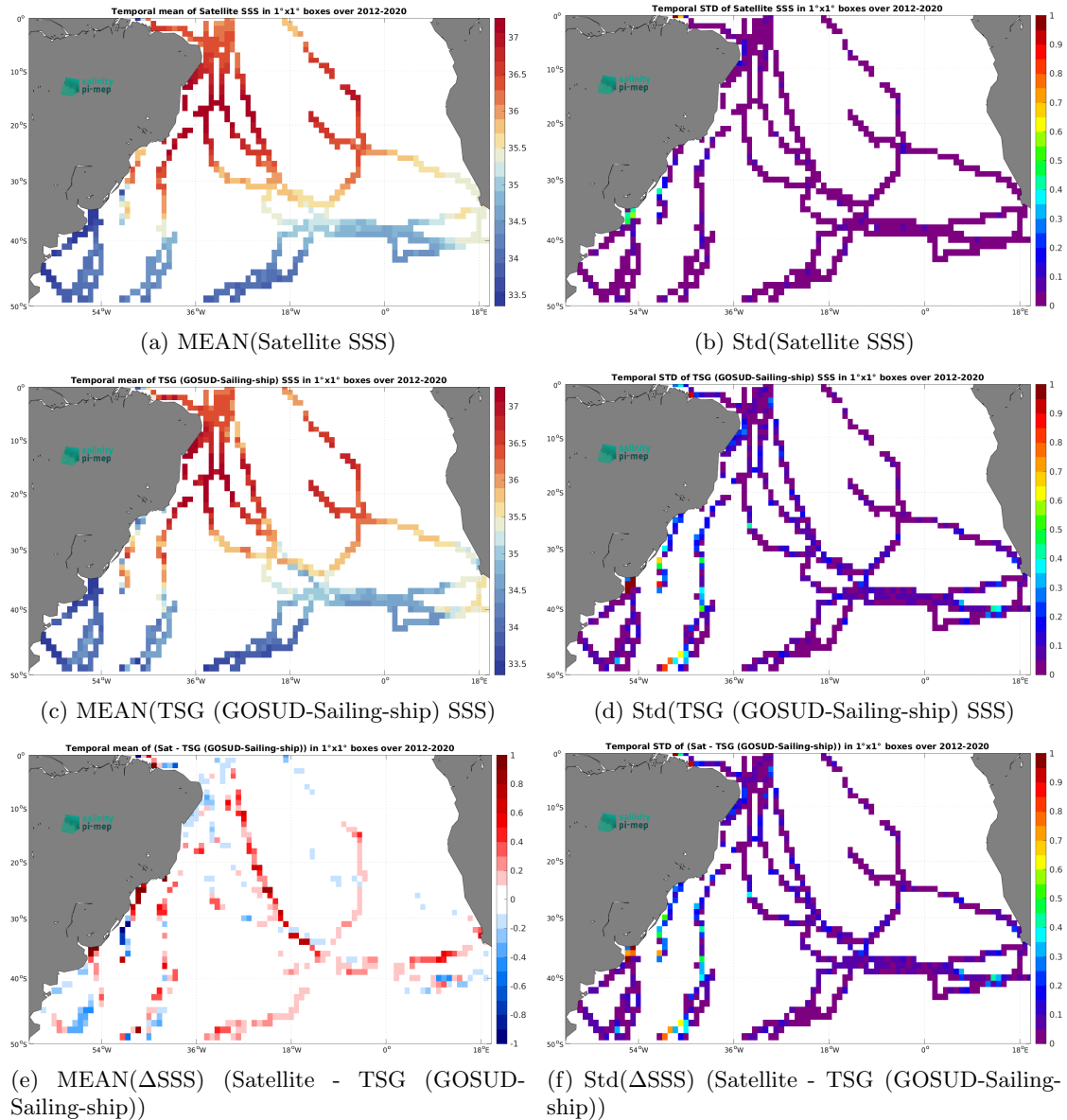
Figure 6: Temporal mean (left) and Std (right) of SSS from SMAP SSS L4 OI v2 - Monthly (IPRC) (top), TSG (GOSUD-Sailing-ship) (middle), and of \Delta SSS (Satellite - TSG (GOSUD-Sailing-ship)). Only match-up pairs are used to generate these maps.
