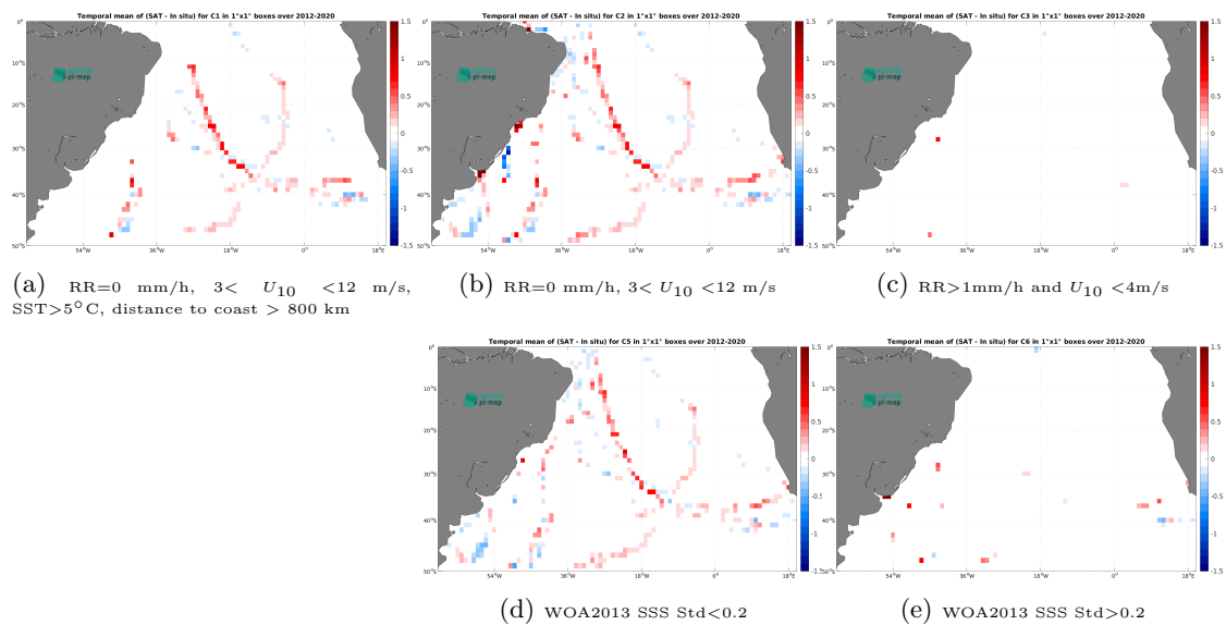
Figure 12: Temporal mean gridded over spatial boxes of size 1^\circ \times 1^\circ of \Delta SSS (SMAP SSS L4 OI v2 - Monthly (IPRC) - TSG (GOSUD-Sailing-ship)) for 5 different subdatasets corresponding to:RR=0 mm/h, 3 < U_{10} < 12 m/s, SST >5^\circ\text{C} , distance to coast > 800 km (a), RR=0 mm/h, 3 < U_{10} < 12 m/s (b), RR >1 mm/h and U_{10} < 4 m/s (c), WOA2013 SSS Std <0.2 (d), WOA2013 SSS Std >0.2 (e).
