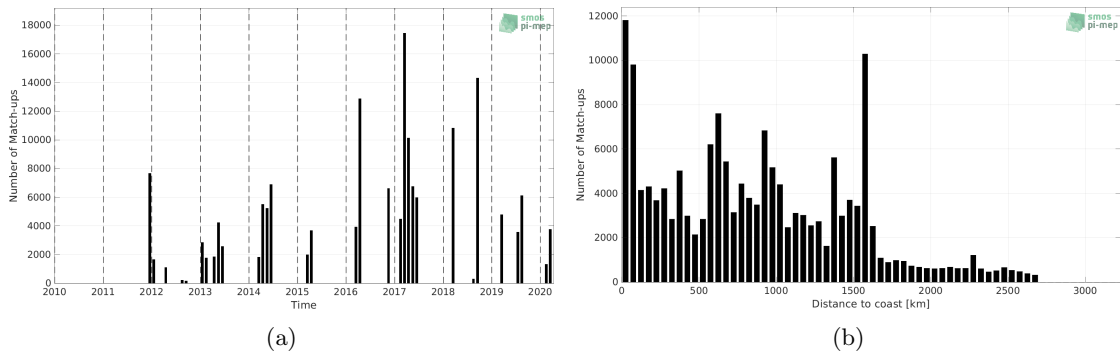
Figure 1: Number of match-ups between TSG (GOSUD-Research-vessel) and SMAP SSS L4 OI v2 - Monthly (IPRC) SSS as a function of time (a) and as function of the distance to coast (b) over the South Atlantic Ocean Pi-MEP region and for the full satellite product period.
