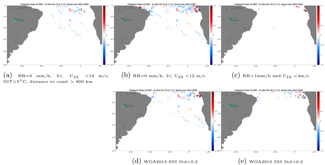
Figure 12: Temporal mean gridded over spatial boxes of size 1^\circ \times 1^\circ of \Delta SSS (SMAP SSS L4 OI v2 - Monthly (IPRC) - TSG (GOSUD-Research-vessel)) for 5 different subdatasets corresponding to:RR=0 mm/h, 3 < U_{10} < 12 m/s, SST>5°C, distance to coast > 800 km (a), RR=0 mm/h, 3 < U_{10} < 12 m/s (b), RR>1mm/h and U_{10} < 4 m/s (c), WOA2013 SSS Std<0.2 (d), WOA2013 SSS Std>0.2 (e).
