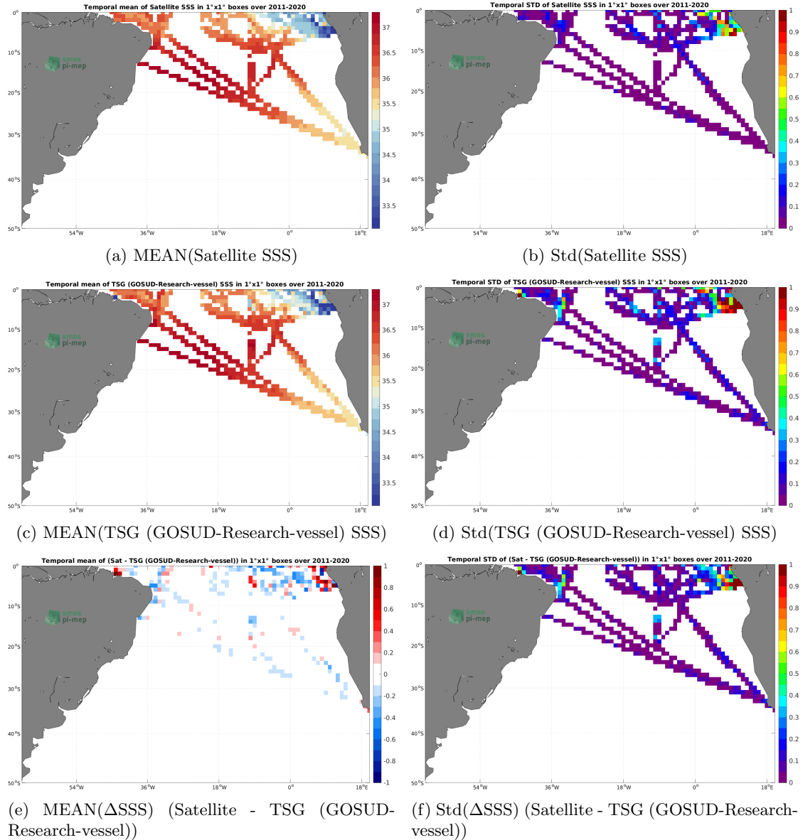
Figure 6: Temporal mean (left) and Std (right) of SSS from SMAP SSS L4 OI v2 - Monthly (IPRC) (top), TSG (GOSUD-Research-vessel) (middle), and of \Delta SSS (Satellite - TSG (GOSUD-Research-vessel)). Only match-up pairs are used to generate these maps.
