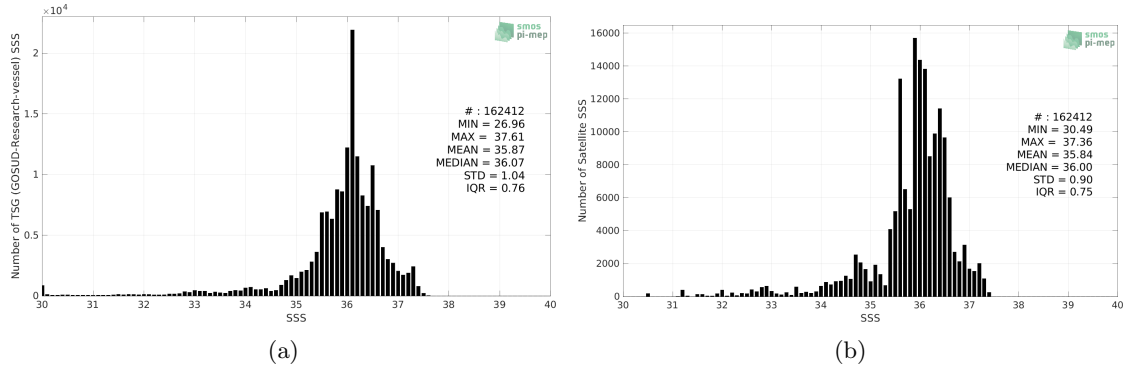
Figure 2: Histograms of SSS from TSG (GOSUD-Research-vessel) (a) and SMAP SSS L4 OI v2 - Monthly (IPRC) (b) considering all match-up pairs per bins of 0.1 over the South Atlantic Ocean Pi-MEP region and for the full satellite product period.
