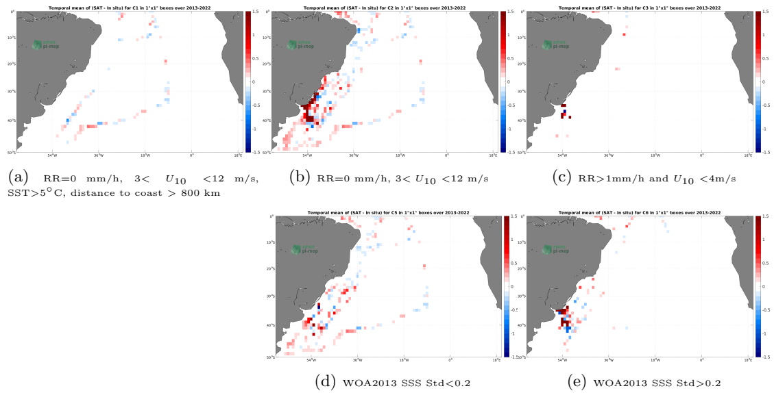
Figure 12: Temporal mean gridded over spatial boxes of size 1^\circ \times 1^\circ of \Delta SSS (SMAP SSS L4 OI v2 - Monthly (IPRC) - TSG (CSIC-UTM)) for 5 different subdatasets corresponding to:RR=0 mm/h, 3 < U_{10} < 12 m/s, SST >5^\circ\text{C} , distance to coast > 800 km (a), RR=0 mm/h, 3 < U_{10} < 12 m/s (b), RR >1 mm/h and U_{10} < 4 m/s (c), WOA2013 SSS Std <0.2 (d), WOA2013 SSS Std >0.2 (e).
