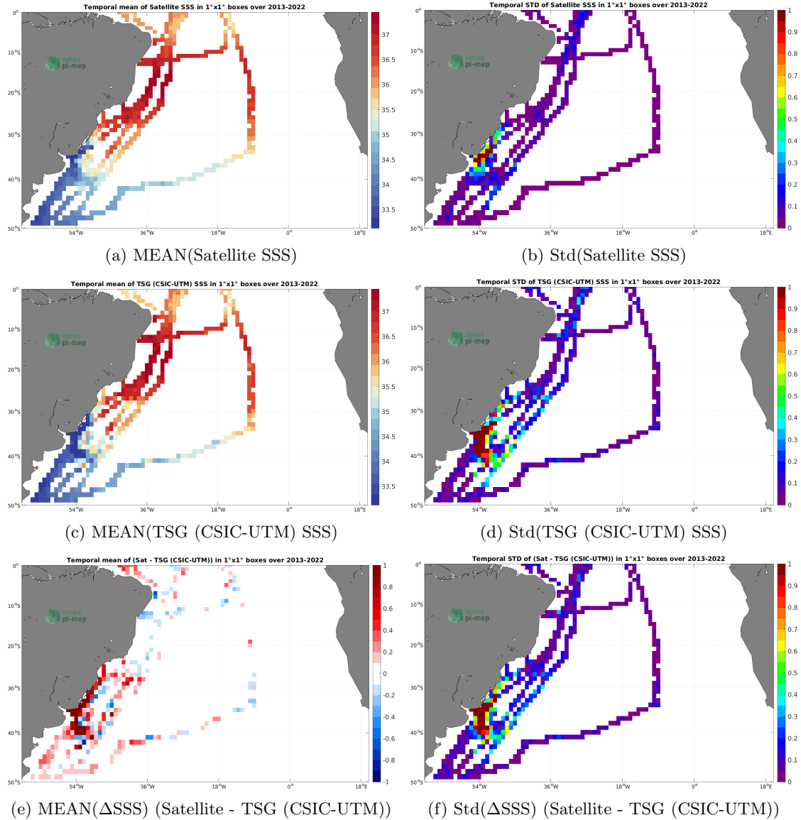
Figure 6: Temporal mean (left) and Std (right) of SSS from SMAP SSS L4 OI v2 - Monthly (IPRC) (top), TSG (CSIC-UTM) (middle), and of \Delta SSS (Satellite - TSG (CSIC-UTM)). Only match-up pairs are used to generate these maps.
