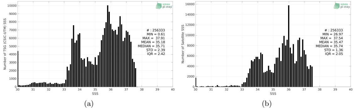
Figure 2: Histograms of SSS from TSG (CSIC-UTM) (a) and SMAP SSS L4 OI v2 - Monthly (IPRC) (b) considering all match-up pairs per bins of 0.1 over the South Atlantic Ocean Pi-MEP region and for the full satellite product period.
