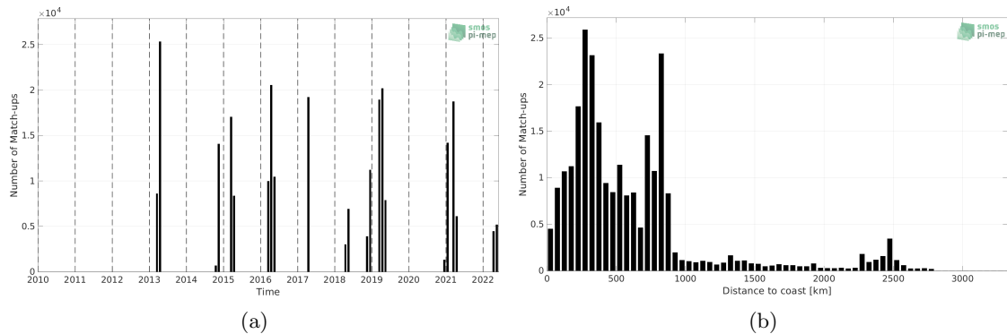
Figure 1: Number of match-ups between TSG (CSIC-UTM) and SMAP SSS L4 OI v2 - Monthly (IPRC) SSS as a function of time (a) and as function of the distance to coast (b) over the South Atlantic Ocean Pi-MEP region and for the full satellite product period.
