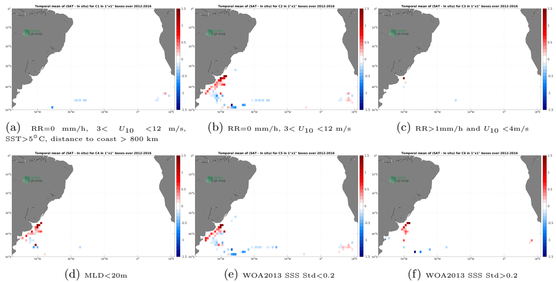
Figure 12: Temporal mean gridded over spatial boxes of size 1^\circ \times 1^\circ of \Delta SSS (SMAP SSS L4 OI v2 - Monthly (IPRC) - Marine mammals) for 6 different subdatasets corresponding to:RR=0 mm/h, 3 < U_{10} < 12 m/s, SST > 5^\circ\text{C} , distance to coast > 800 km (a), RR=0 mm/h, 3 < U_{10} < 12 m/s (b), RR > 1 mm/h and U_{10} < 4 m/s (c),MLD < 20 m (d),WOA2013 SSS Std < 0.2 (e),WOA2013 SSS Std > 0.2 (f).
