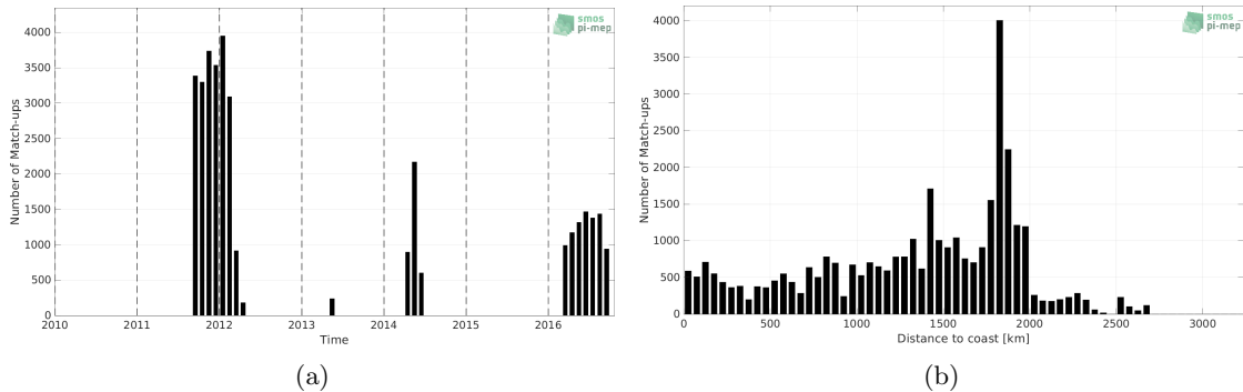
Figure 1: Number of match-ups between Surface drifters and SMAP SSS L4 OI v2 - Monthly (IPRC) SSS as a function of time (a) and as function of the distance to coast (b) over the South Atlantic Ocean Pi-MEP region and for the full satellite product period.
