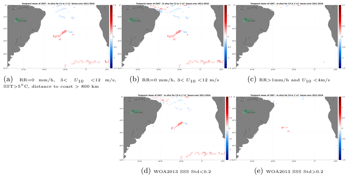
Figure 11: Temporal mean gridded over spatial boxes of size 1^\circ \times 1^\circ of \Delta SSS (SMAP SSS L4 OI v2 - Monthly (IPRC) - Surface drifters) for 5 different subdatasets corresponding to:RR=0 mm/h, 3 < U_{10} < 12 m/s, SST >5^\circ\text{C} , distance to coast > 800 km (a), RR=0 mm/h, 3 < U_{10} < 12 m/s (b), RR >1 mm/h and U_{10} < 4 m/s (c), WOA2013 SSS Std <0.2 (d), WOA2013 SSS Std >0.2 (e).
