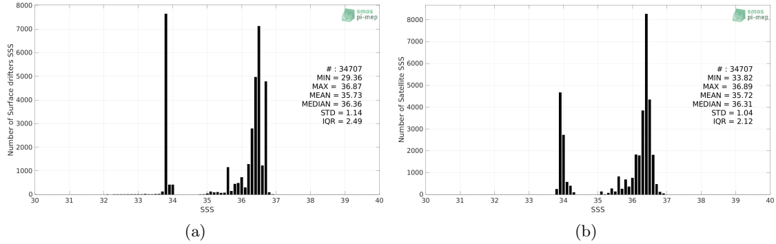
Figure 2: Histograms of SSS from Surface drifters (a) and SMAP SSS L4 OI v2 - Monthly (IPRC) (b) considering all match-up pairs per bins of 0.1 over the South Atlantic Ocean Pi-MEP region and for the full satellite product period.
