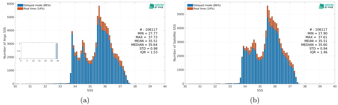
Figure 2: Histograms of SSS from Argo (a) and SMAP SSS L4 OI v2 - Monthly (IPRC) (b) considering all match-up pairs per bins of 0.1 over the South Atlantic Ocean Pi-MEP region and for the full satellite product period.
