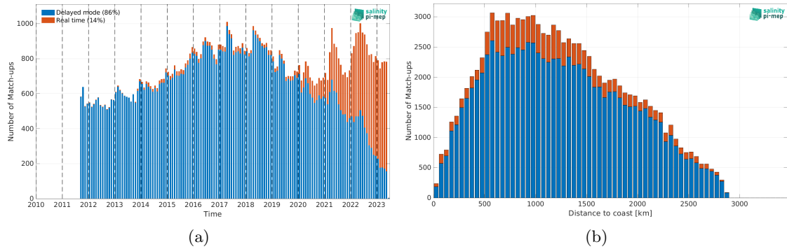
Figure 1: Number of match-ups between Argo and SMAP SSS L4 OI v2 - Monthly (IPRC) SSS as a function of time (a) and as function of the distance to coast (b) over the South Atlantic Ocean Pi-MEP region and for the full satellite product period.
