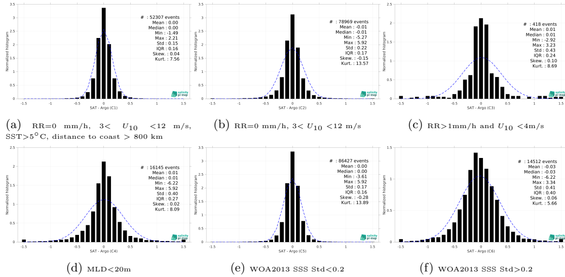
Figure 13: Normalized histogram of \Delta SSS (SMAP SSS L4 OI v2 - Monthly (IPRC) - Argo) for 6 different subdatasets corresponding to: RR=0 mm/h, 3 < U_{10} < 12 m/s, SST > 5°C, distance to coast > 800 km (a), RR=0 mm/h, 3 < U_{10} < 12 m/s (b), RR > 1mm/h and U_{10} < 4 m/s (c), MLD < 20m (d), WOA2013 SSS Std < 0.2 (e), WOA2013 SSS Std > 0.2 (f).
