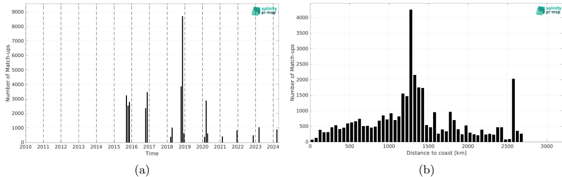
Figure 2: Number of match-ups between TSG (SAMOS) and SMAP SSS L3 v6 - 8-Day running (RSS) SSS as a function of time (a) and as function of the distance to coast (b) over the South Atlantic Ocean Pi-MEP region and for the full satellite product period.
