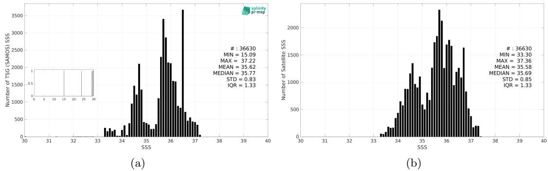
Figure 3: Histograms of SSS from TSG (SAMOS) (a) and SMAP SSS L3 v6 - 8-Day running (RSS) (b) considering all match-up pairs per bins of 0.1 over the South Atlantic Ocean Pi-MEP region and for the full satellite product period.
