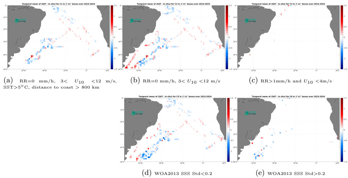
Figure 14: Temporal mean gridded over spatial boxes of size 1^\circ \times 1^\circ of \Delta\text{SSS} (SMAP SSS L3 v6 - 8-Day running (RSS) - TSG (SAMOS)) for 5 different subdatasets corresponding to:RR=0 mm/h, 3 < U_{10} < 12 m/s, SST >5^\circ\text{C} , distance to coast > 800 km (a), RR=0 mm/h, 3 < U_{10} < 12 m/s (b), RR >1 mm/h and U_{10} < 4 m/s (c), WOA2013 SSS Std <0.2 (d), WOA2013 SSS Std >0.2 (e).
