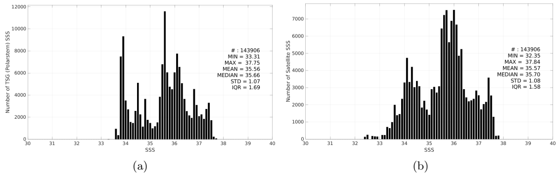
Figure 3: Histograms of SSS from TSG (Polarstern) (a) and SMAP SSS L3 v6 - 8-Day running (RSS) (b) considering all match-up pairs per bins of 0.1 over the South Atlantic Ocean Pi-MEP region and for the full satellite product period.
