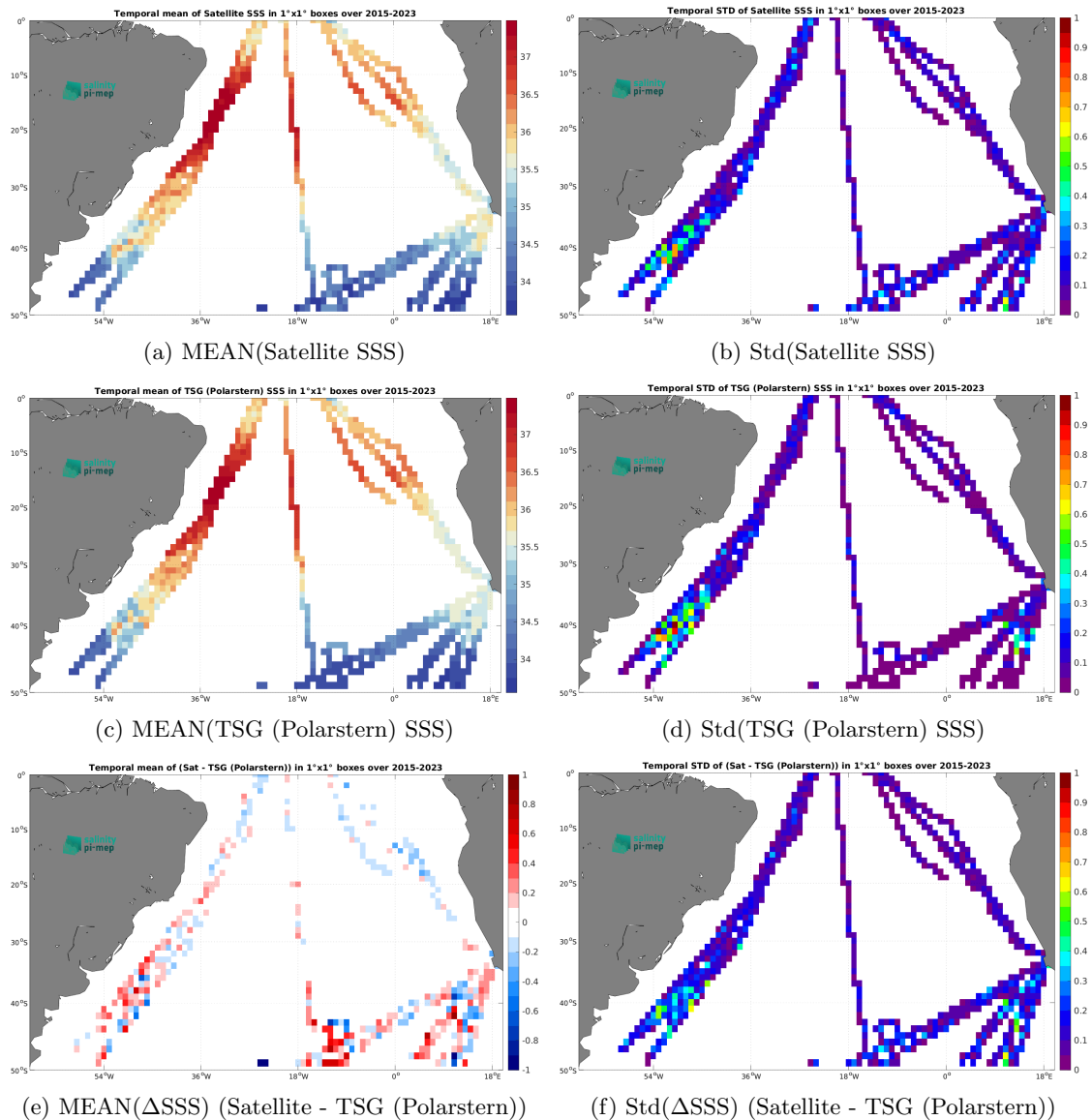
Figure 7: Temporal mean (left) and Std (right) of SSS from SMAP SSS L3 v6 - 8-Day running (RSS) (top), TSG (Polarstern) (middle), and of \Delta SSS (Satellite - TSG (Polarstern)). Only match-up pairs are used to generate these maps.
