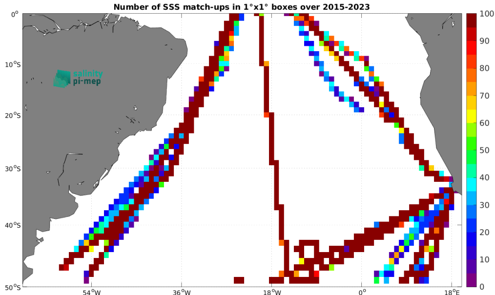
Figure 5: Number of SSS match-ups between TSG (Polarstern) SSS and the SMAP SSS L3 v6 - 8-Day running (RSS) SSS product for the South Atlantic Ocean Pi-MEP region over 1^\circ \times 1^\circ boxes and for the full satellite product period.
