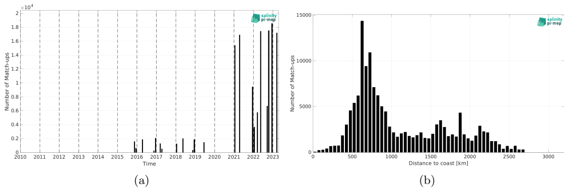
Figure 2: Number of match-ups between TSG (Polarstern) and SMAP SSS L3 v6 - 8-Day running (RSS) SSS as a function of time (a) and as function of the distance to coast (b) over the South Atlantic Ocean Pi-MEP region and for the full satellite product period.
