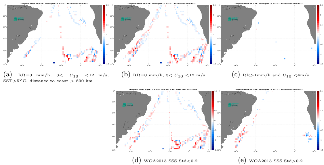
Figure 14: Temporal mean gridded over spatial boxes of size 1^\circ \times 1^\circ of \Delta\text{SSS} (SMAP SSS L3 v6 - 8-Day running (RSS) - TSG (Polarstern)) for 5 different subdatasets corresponding to:RR=0 mm/h, 3 < U_{10} < 12 m/s, SST >5^\circ\text{C} , distance to coast > 800 km (a), RR=0 mm/h, 3 < U_{10} < 12 m/s (b), RR >1 mm/h and U_{10} < 4 m/s (c), WOA2013 SSS Std <0.2 (d), WOA2013 SSS Std >0.2 (e).
