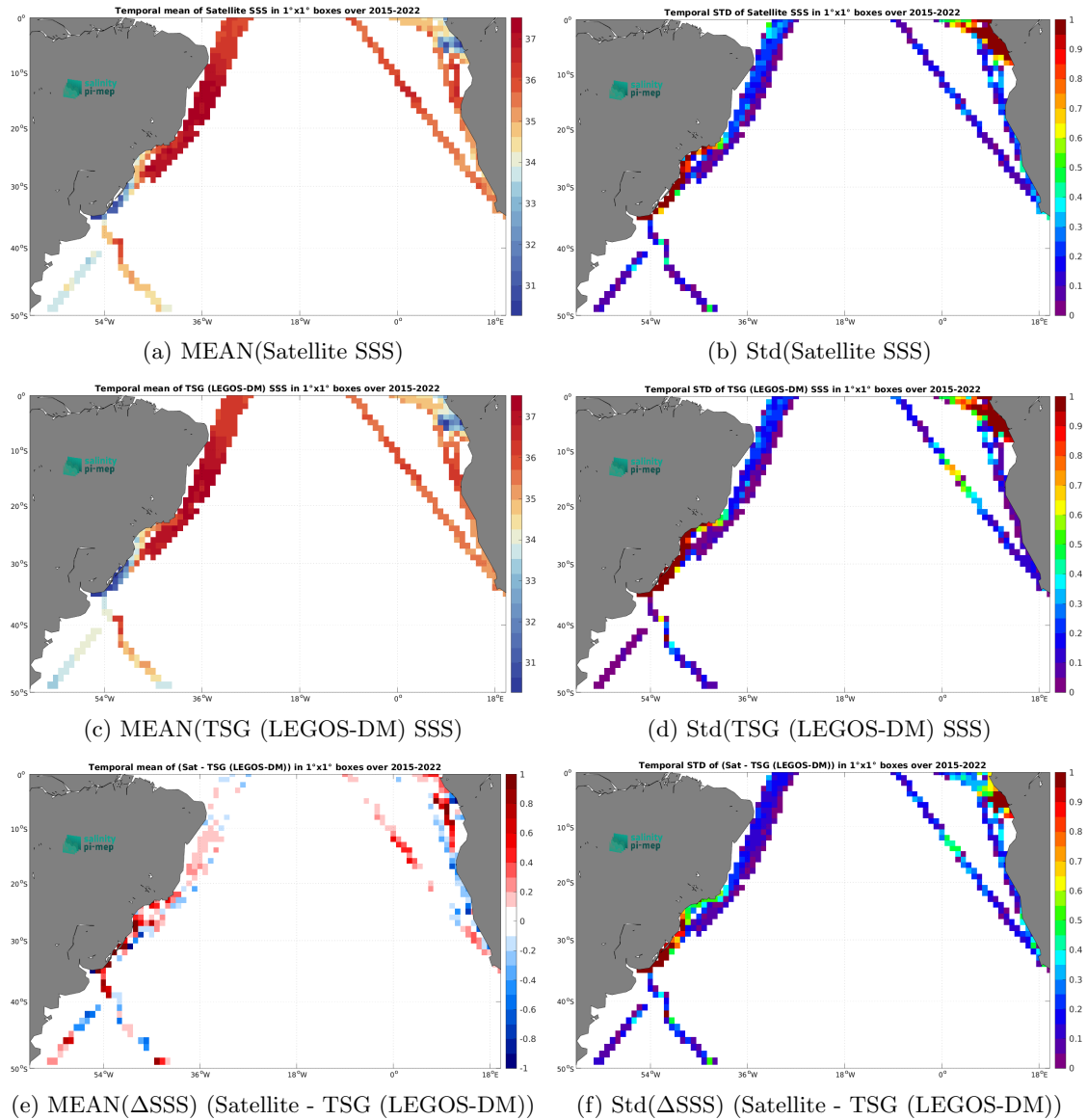
Figure 7: Temporal mean (left) and Std (right) of SSS from SMAP SSS L3 v6 - 8-Day running (RSS) (top), TSG (LEGOS-DM) (middle), and of \Delta SSS (Satellite - TSG (LEGOS-DM)). Only match-up pairs are used to generate these maps.
