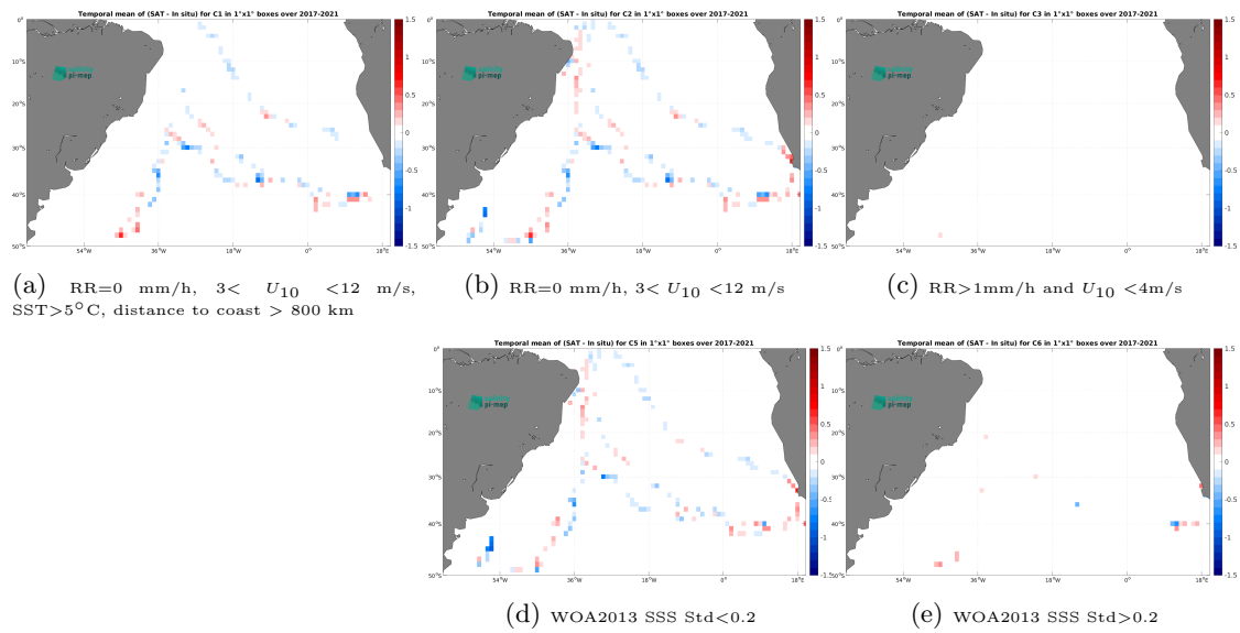
Figure 14: Temporal mean gridded over spatial boxes of size 1^\circ \times 1^\circ of \Delta\text{SSS} (SMAP SSS L3 v6 - 8-Day running (RSS) - TSG (GOSUD-Sailing-ship)) for 5 different subdatasets corresponding to:RR=0 mm/h, 3 < U_{10} < 12 m/s, SST >5^\circ\text{C} , distance to coast > 800 km (a), RR=0 mm/h, 3 < U_{10} < 12 m/s (b), RR >1 mm/h and U_{10} < 4 m/s (c), WOA2013 SSS Std <0.2 (d), WOA2013 SSS Std >0.2 (e).
