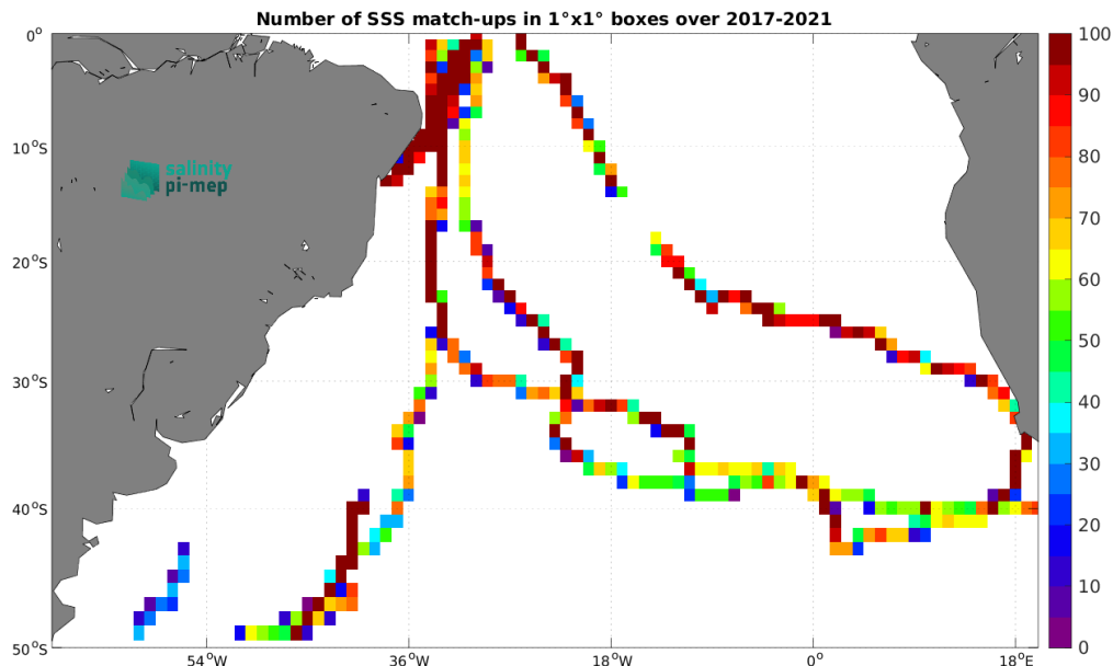
Figure 5: Number of SSS match-ups between TSG (GOSUD-Sailing-ship) SSS and the SMAP SSS L3 v6 - 8-Day running (RSS) SSS product for the South Atlantic Ocean Pi-MEP region over 1^\circ \times 1^\circ boxes and for the full satellite product period.
