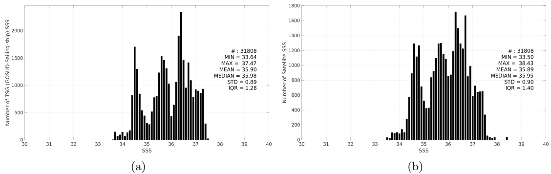
Figure 3: Histograms of SSS from TSG (GOSUD-Sailing-ship) (a) and SMAP SSS L3 v6 - 8-Day running (RSS) (b) considering all match-up pairs per bins of 0.1 over the South Atlantic Ocean Pi-MEP region and for the full satellite product period.
