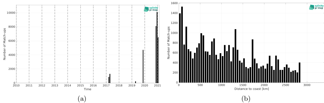
Figure 2: Number of match-ups between TSG (GOSUD-Sailing-ship) and SMAP SSS L3 v6 - 8-Day running (RSS) SSS as a function of time (a) and as function of the distance to coast (b) over the South Atlantic Ocean Pi-MEP region and for the full satellite product period.
