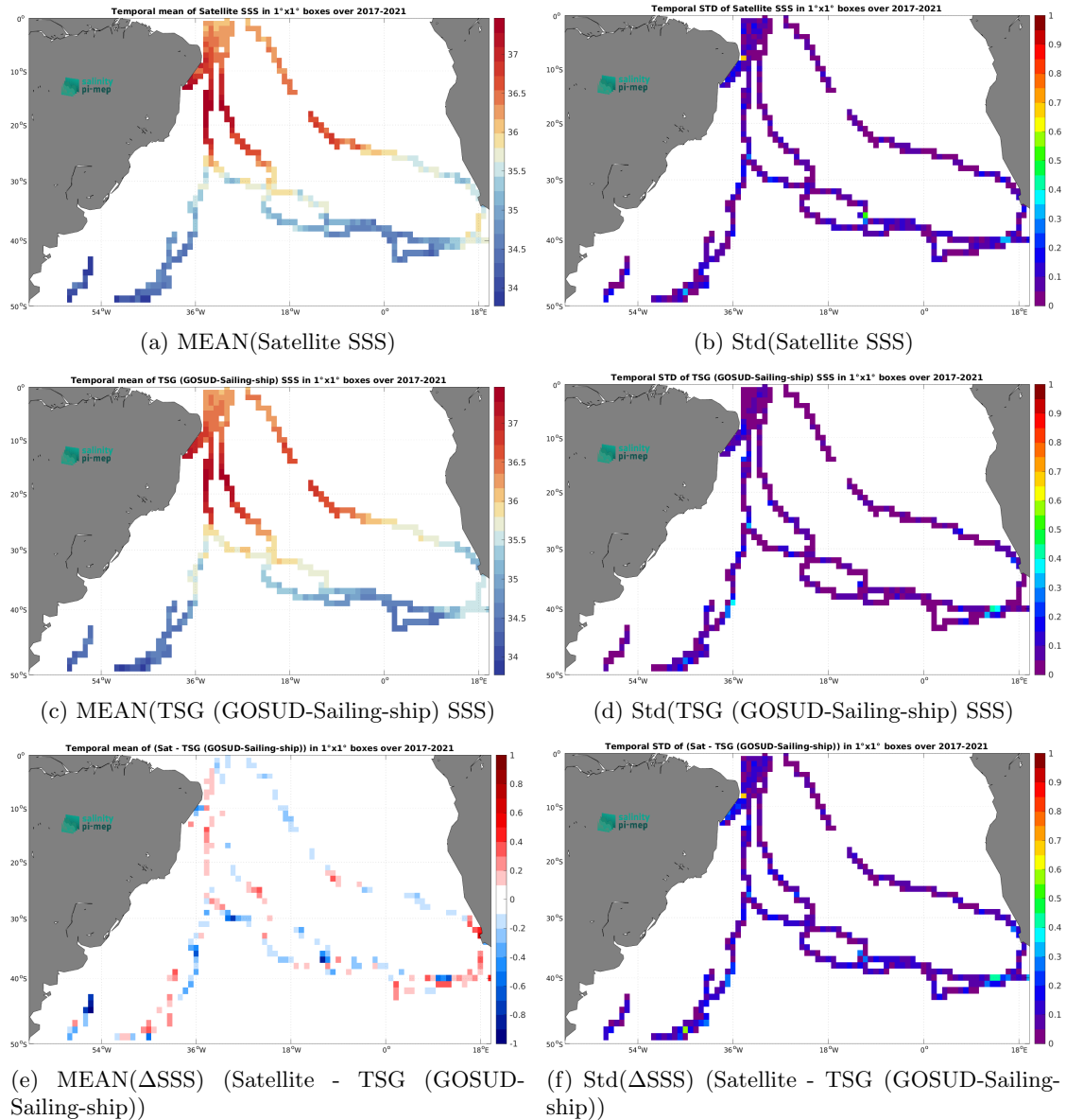
Figure 7: Temporal mean (left) and Std (right) of SSS from SMAP SSS L3 v6 - 8-Day running (RSS) (top), TSG (GOSUD-Sailing-ship) (middle), and of \Delta SSS (Satellite - TSG (GOSUD-Sailing-ship)). Only match-up pairs are used to generate these maps.
