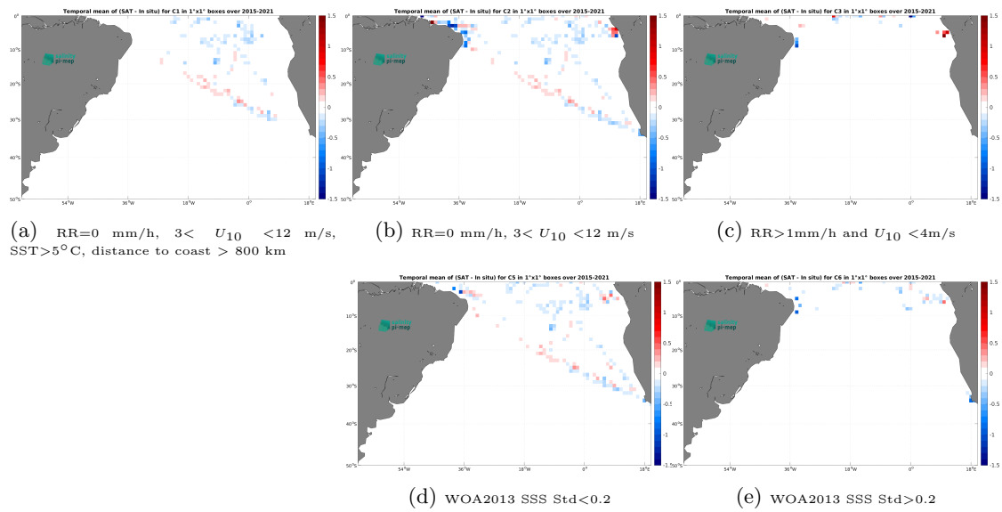
Figure 14: Temporal mean gridded over spatial boxes of size 1^\circ \times 1^\circ of \Delta\text{SSS} (SMAP SSS L3 v6 - 8-Day running (RSS) - TSG (GOSUD-Research-vessel)) for 5 different subdatasets corresponding to:RR=0 mm/h, 3 < U_{10} < 12 m/s, SST >5^\circ\text{C} , distance to coast > 800 km (a), RR=0 mm/h, 3 < U_{10} < 12 m/s (b), RR >1 mm/h and U_{10} < 4 m/s (c), WOA2013 SSS Std <0.2 (d), WOA2013 SSS Std >0.2 (e).
