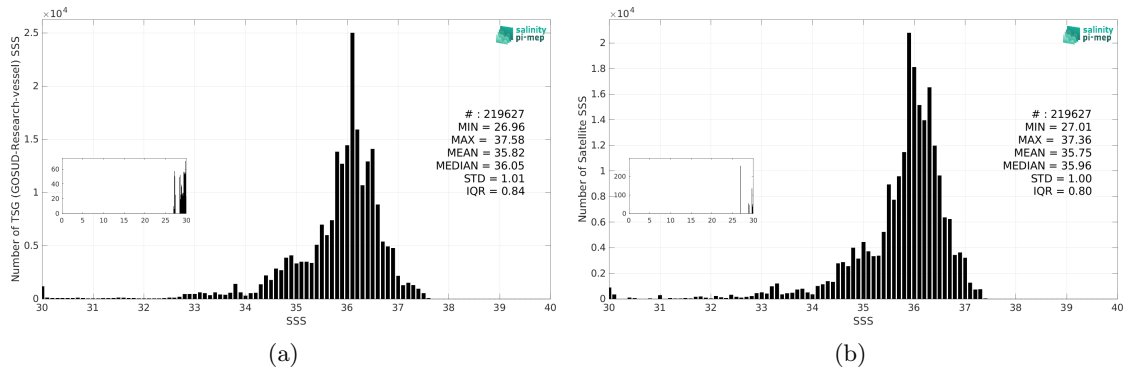
Figure 3: Histograms of SSS from TSG (GOSUD-Research-vessel) (a) and SMAP SSS L3 v6 - 8-Day running (RSS) (b) considering all match-up pairs per bins of 0.1 over the South Atlantic Ocean Pi-MEP region and for the full satellite product period.
