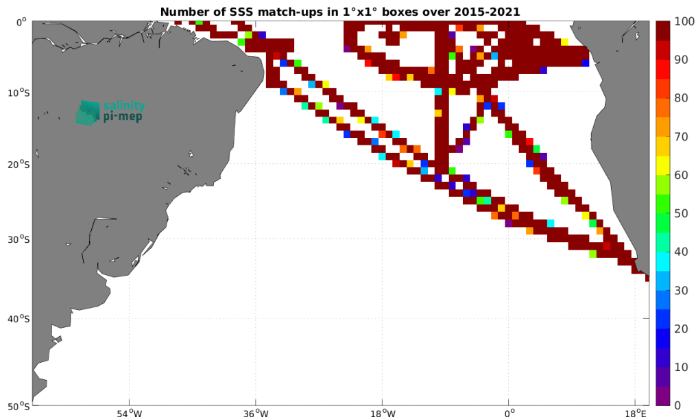
Figure 5: Number of SSS match-ups between TSG (GOSUD-Research-vessel) SSS and the SMAP SSS L3 v6 - 8-Day running (RSS) SSS product for the South Atlantic Ocean Pi-MEP region over 1^\circ \times 1^\circ boxes and for the full satellite product period.
