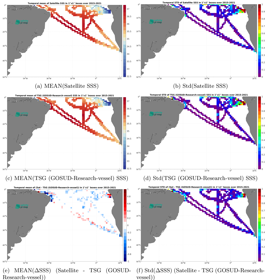
Figure 7: Temporal mean (left) and Std (right) of SSS from SMAP SSS L3 v6 - 8-Day running (RSS) (top), TSG (GOSUD-Research-vessel) (middle), and of \Delta SSS (Satellite - TSG (GOSUD-Research-vessel)). Only match-up pairs are used to generate these maps.
