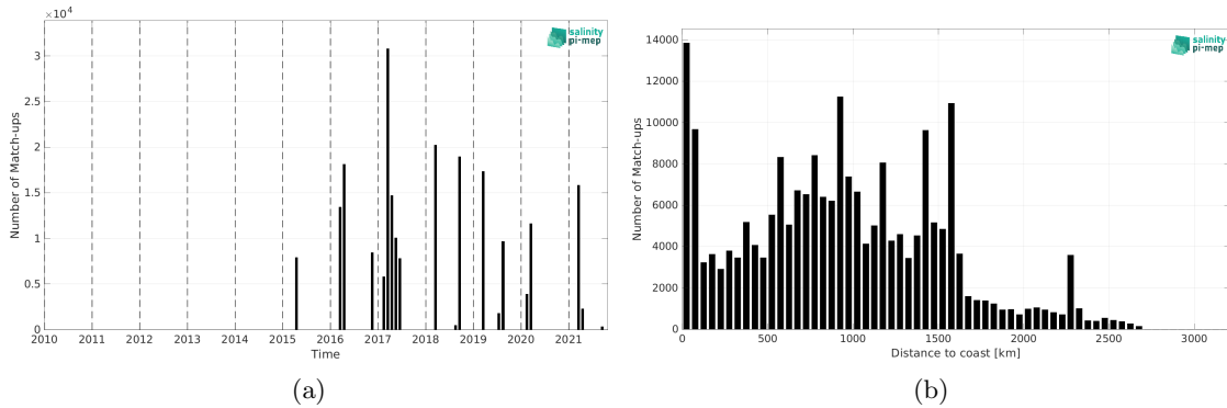
Figure 2: Number of match-ups between TSG (GOSUD-Research-vessel) and SMAP SSS L3 v6 - 8-Day running (RSS) SSS as a function of time (a) and as function of the distance to coast (b) over the South Atlantic Ocean Pi-MEP region and for the full satellite product period.
