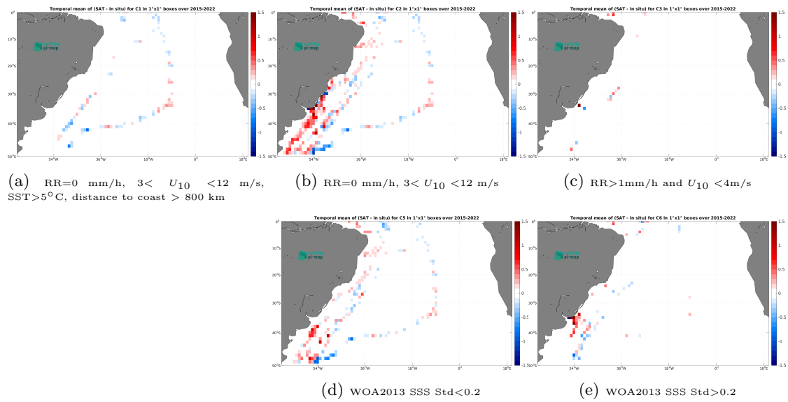
Figure 14: Temporal mean gridded over spatial boxes of size 1^\circ \times 1^\circ of \Delta\text{SSS} (SMAP SSS L3 v6 - 8-Day running (RSS) - TSG (CSIC-UTM)) for 5 different subdatasets corresponding to:RR=0 mm/h, 3 < U_{10} < 12 m/s, SST > 5^\circ\text{C} , distance to coast > 800 km (a), RR=0 mm/h, 3 < U_{10} < 12 m/s (b), RR > 1 mm/h and U_{10} < 4 m/s (c), WOA2013 SSS Std < 0.2 (d), WOA2013 SSS Std > 0.2 (e).
