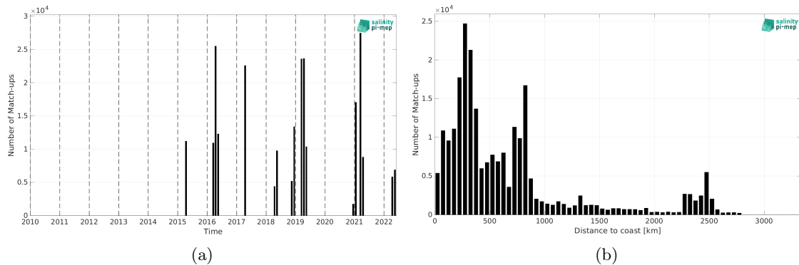
Figure 2: Number of match-ups between TSG (CSIC-UTM) and SMAP SSS L3 v6 - 8-Day running (RSS) SSS as a function of time (a) and as function of the distance to coast (b) over the South Atlantic Ocean Pi-MEP region and for the full satellite product period.
