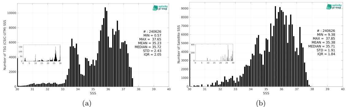
Figure 3: Histograms of SSS from TSG (CSIC-UTM) (a) and SMAP SSS L3 v6 - 8-Day running (RSS) (b) considering all match-up pairs per bins of 0.1 over the South Atlantic Ocean Pi-MEP region and for the full satellite product period.
