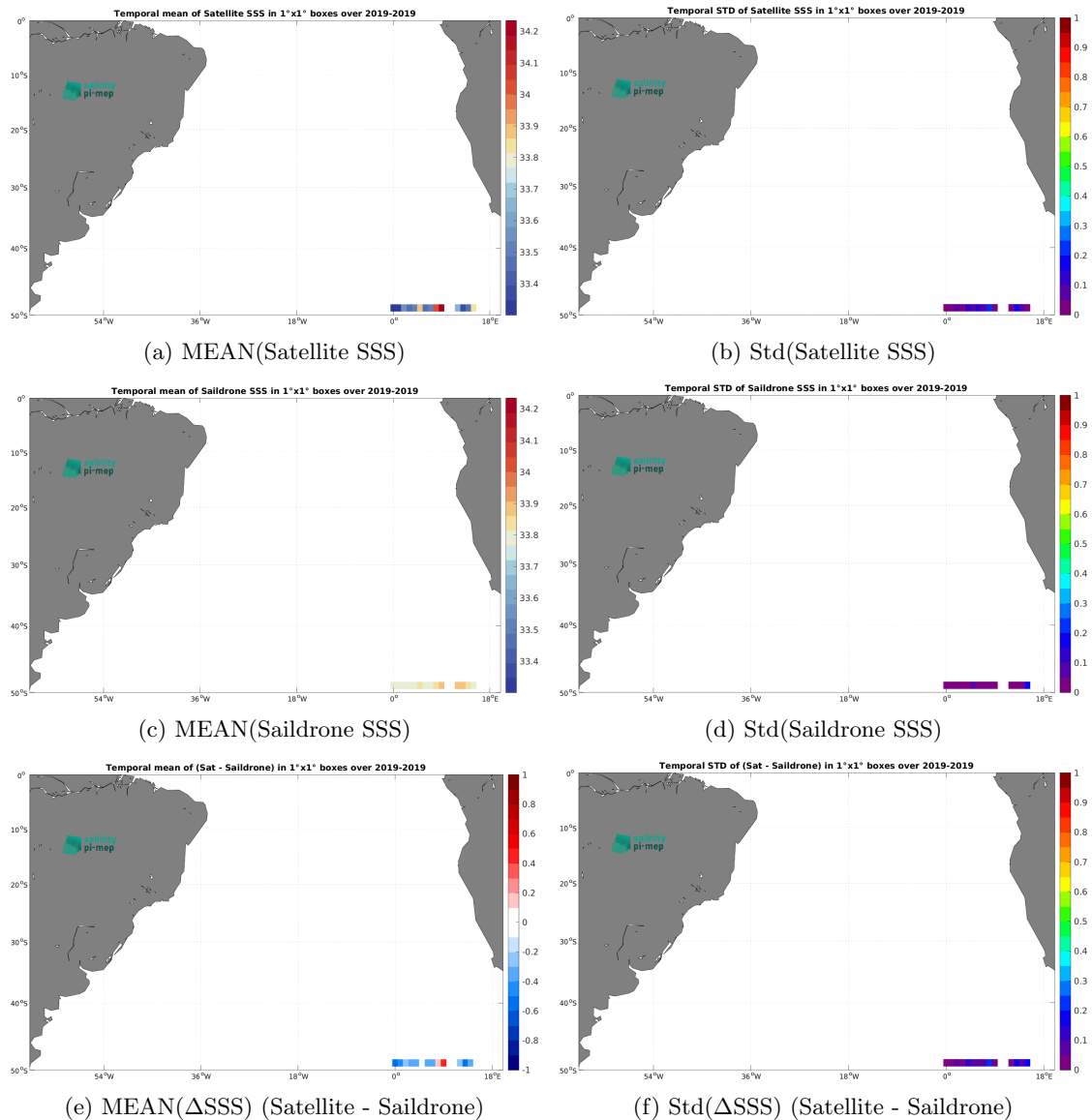
Figure 7: Temporal mean (left) and Std (right) of SSS from SMAP SSS L3 v6 - 8-Day running (RSS) (top), Saildrone (middle), and of \Delta SSS (Satellite - Saildrone). Only match-up pairs are used to generate these maps.
