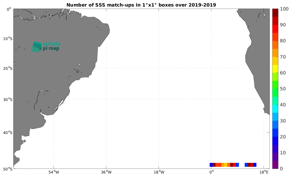
Figure 5: Number of SSS match-ups between Saildrone SSS and the SMAP SSS L3 v6 - 8-Day running (RSS) SSS product for the South Atlantic Ocean Pi-MEP region over 1^\circ \times 1^\circ boxes and for the full satellite product period.
