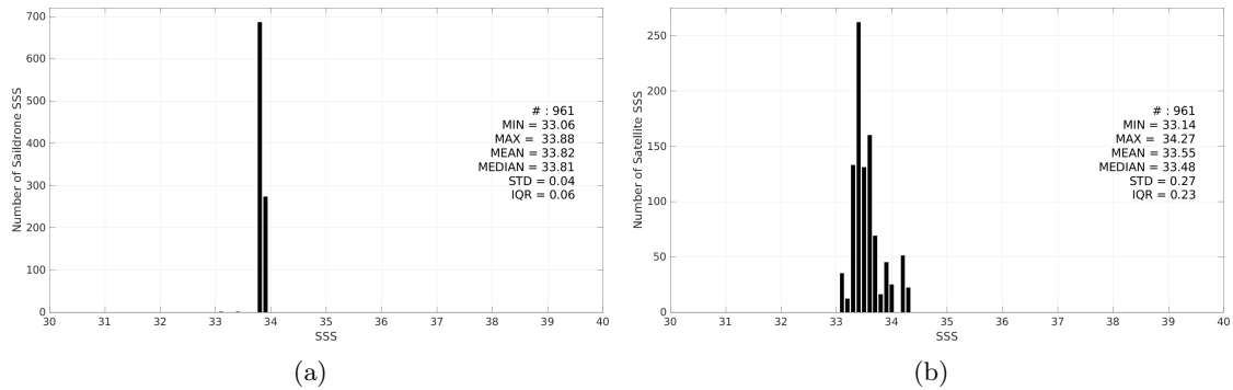
Figure 3: Histograms of SSS from Saildrone (a) and SMAP SSS L3 v6 - 8-Day running (RSS) (b) considering all match-up pairs per bins of 0.1 over the South Atlantic Ocean Pi-MEP region and for the full satellite product period.
