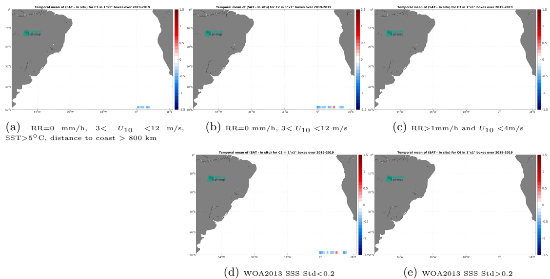
Figure 14: Temporal mean gridded over spatial boxes of size 1^\circ \times 1^\circ of \Delta SSS (SMAP SSS L3 v6 - 8-Day running (RSS) - Saildrone) for 5 different subdatasets corresponding to:RR=0 mm/h, 3 < U_{10} < 12 m/s, SST >5^\circ\text{C} , distance to coast > 800 km (a), RR=0 mm/h, 3 < U_{10} < 12 m/s (b), RR >1 mm/h and U_{10} < 4 m/s (c), WOA2013 SSS Std <0.2 (d), WOA2013 SSS Std >0.2 (e).
