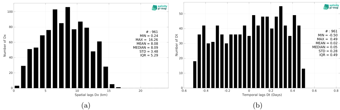
Figure 6: Histograms of the spatial (a) and temporal (b) lags between the location/time of the Saildrone measurement and the date of the corresponding SMAP SSS L3 v6 - 8-Day running (RSS) SSS pixel.
