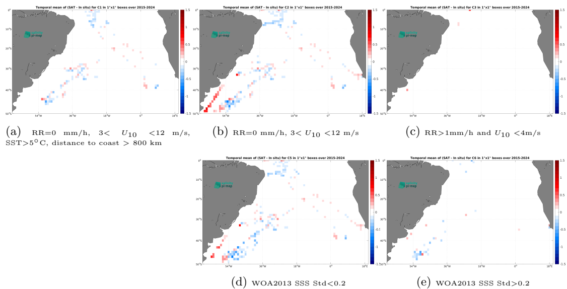
Figure 14: Temporal mean gridded over spatial boxes of size 1^\circ \times 1^\circ of \Delta\text{SSS} (SMAP SSS L3 v6 - Monthly (RSS) - TSG (SAMOS)) for 5 different subdatasets corresponding to:RR=0 mm/h, 3 < U_{10} < 12 m/s, SST >5^\circ\text{C} , distance to coast > 800 km (a), RR=0 mm/h, 3 < U_{10} < 12 m/s (b), RR >1 mm/h and U_{10} < 4 m/s (c), WOA2013 SSS Std <0.2 (d), WOA2013 SSS Std >0.2 (e).
