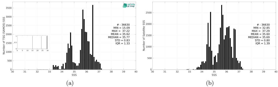
Figure 3: Histograms of SSS from TSG (SAMOS) (a) and SMAP SSS L3 v6 - Monthly (RSS) (b) considering all match-up pairs per bins of 0.1 over the South Atlantic Ocean Pi-MEP region and for the full satellite product period.
