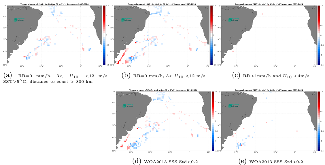
Figure 14: Temporal mean gridded over spatial boxes of size 1^\circ \times 1^\circ of \Delta\text{SSS} (SMAP SSS L3 v6 - Monthly (RSS) - TSG (SAMOS)) for 5 different subdatasets corresponding to:RR=0 mm/h, 3 < U_{10} < 12 m/s, SST >5^\circ\text{C} , distance to coast > 800 km (a), RR=0 mm/h, 3 < U_{10} < 12 m/s (b), RR >1 mm/h and U_{10} < 4 m/s (c), WOA2013 SSS Std <0.2 (d), WOA2013 SSS Std >0.2 (e).
