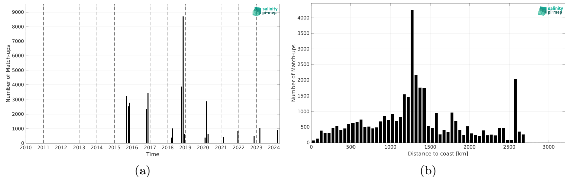
Figure 2: Number of match-ups between TSG (SAMOS) and SMAP SSS L3 v6 - Monthly (RSS) SSS as a function of time (a) and as function of the distance to coast (b) over the South Atlantic Ocean Pi-MEP region and for the full satellite product period.
