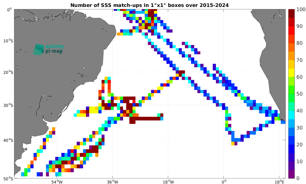
Figure 5: Number of SSS match-ups between TSG (SAMOS) SSS and the SMAP SSS L3 v6 - Monthly (RSS) SSS product for the South Atlantic Ocean Pi-MEP region over 1^\circ \times 1^\circ boxes and for the full satellite product period.
