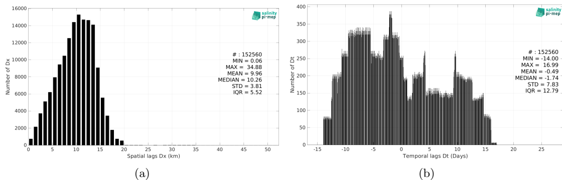
Figure 6: Histograms of the spatial (a) and temporal (b) lags between the location/time of the TSG (Polarstern) measurement and the date of the corresponding SMAP SSS L3 v6 - Monthly (RSS) SSS pixel.
