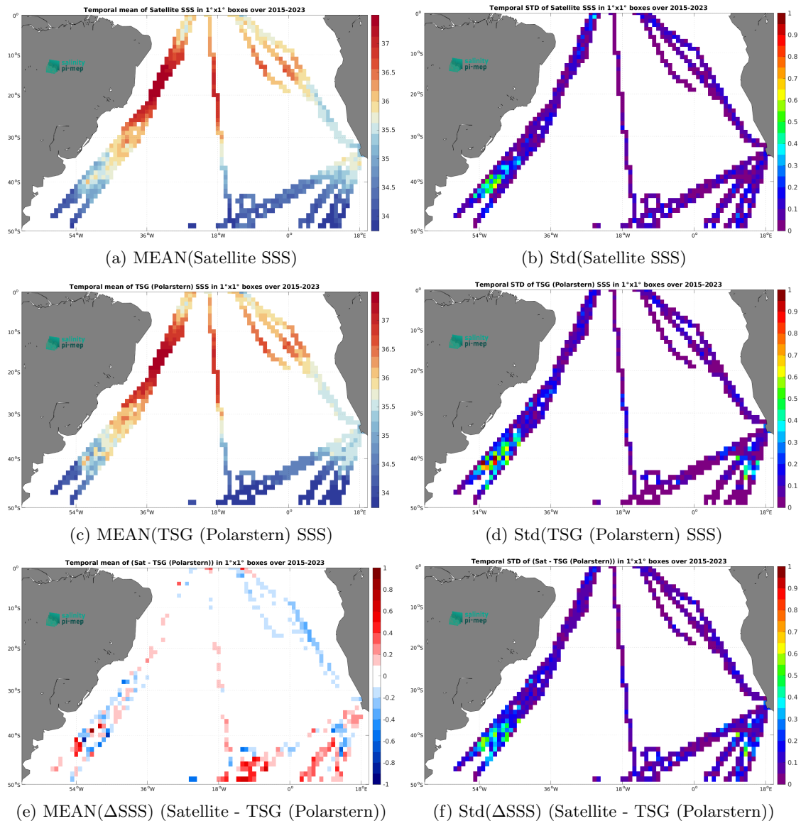
Figure 7: Temporal mean (left) and Std (right) of SSS from SMAP SSS L3 v6 - Monthly (RSS) (top), TSG (Polarstern) (middle), and of \Delta SSS (Satellite - TSG (Polarstern)). Only match-up pairs are used to generate these maps.
