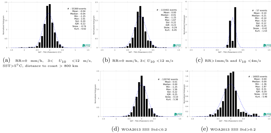
Figure 15: Normalized histogram of \Delta SSS (SMAP SSS L3 v6 - Monthly (RSS) - TSG (Polarstern)) for 5 different subdatasets corresponding to: RR=0 mm/h, 3 < U_{10} < 12 m/s, SST>5°C, distance to coast > 800 km (a), RR=0 mm/h, 3 < U_{10} < 12 m/s (b), RR>1mm/h and U_{10} < 4 m/s (c), WOA2013 SSS Std<0.2 (d), WOA2013 SSS Std>0.2 (e).
