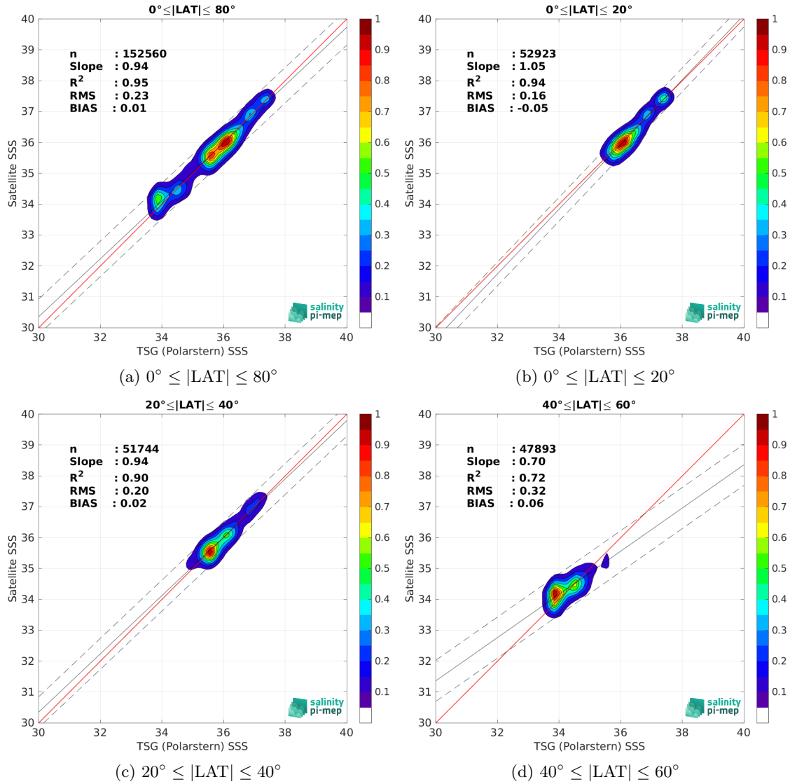
Figure 10: Contour maps of the concentration of SMAP SSS L3 v6 - Monthly (RSS) SSS (y-axis) versus TSG (Polarstern) SSS (x-axis) at match-up pairs for different latitude bands. For each plot, the red line shows x=y . The black thin and dashed lines indicate a linear fit through the data cloud and the \pm 95\% confidence levels, respectively. The number match-up pairs n , the slope and R^2 coefficient of the linear fit, the root mean square (RMS) and the mean bias between satellite and in situ data are indicated for each latitude band in each plots.
