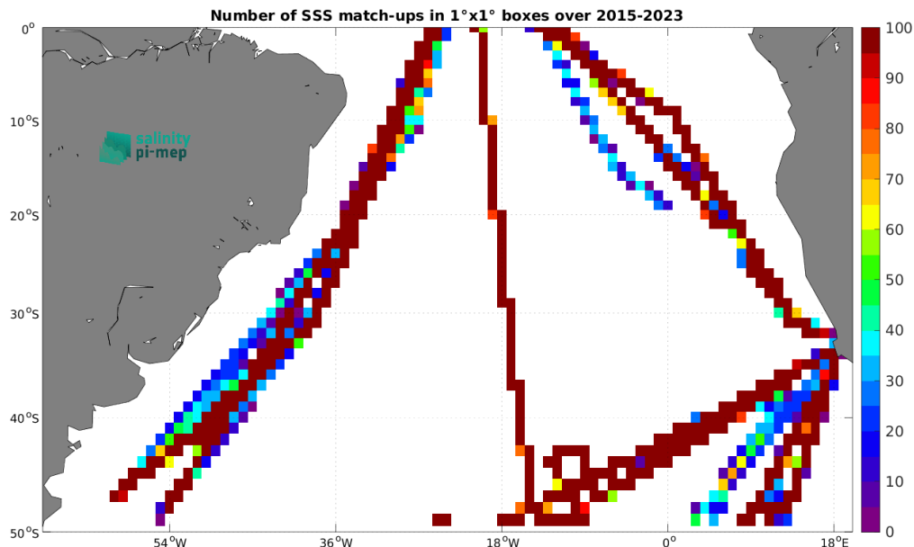
Figure 5: Number of SSS match-ups between TSG (Polarstern) SSS and the SMAP SSS L3 v6 - Monthly (RSS) SSS product for the South Atlantic Ocean Pi-MEP region over 1^\circ \times 1^\circ boxes and for the full satellite product period.
