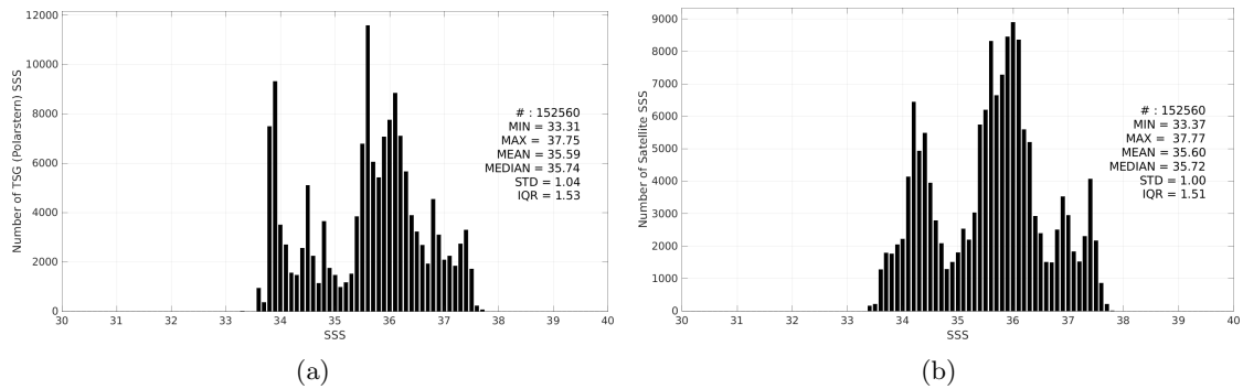
Figure 3: Histograms of SSS from TSG (Polarstern) (a) and SMAP SSS L3 v6 - Monthly (RSS) (b) considering all match-up pairs per bins of 0.1 over the South Atlantic Ocean Pi-MEP region and for the full satellite product period.
