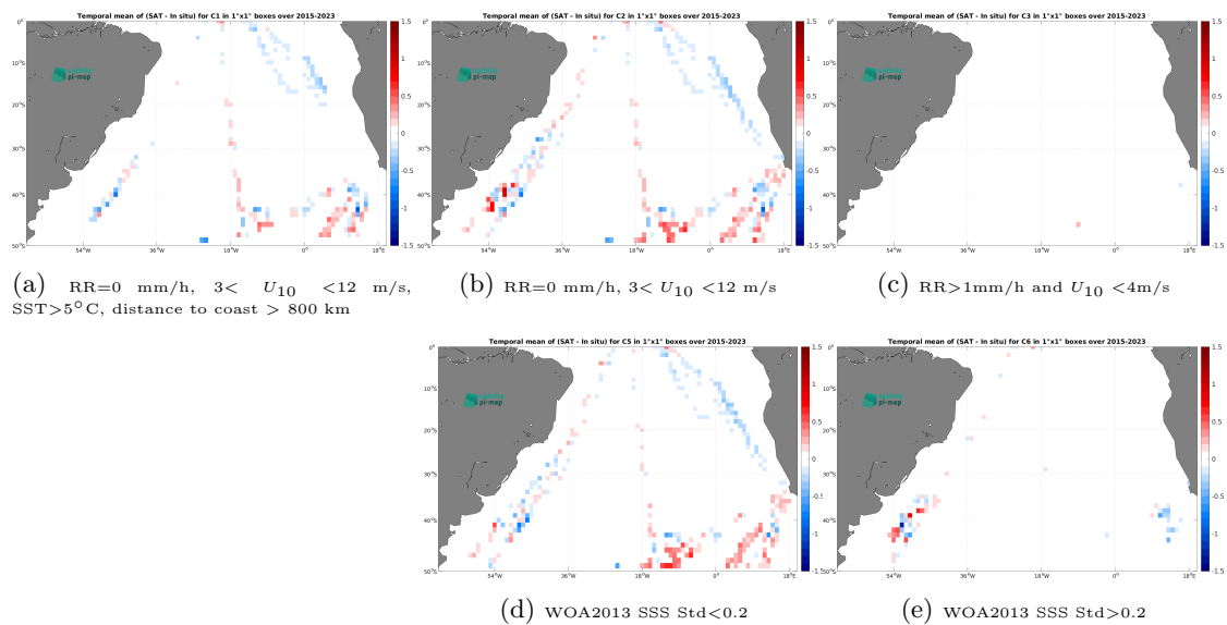
Figure 14: Temporal mean gridded over spatial boxes of size 1^\circ \times 1^\circ of \Delta\text{SSS} (SMAP SSS L3 v6 - Monthly (RSS) - TSG (Polarstern)) for 5 different subdatasets corresponding to:RR=0 mm/h, 3 < U_{10} < 12 m/s, SST >5^\circ\text{C} , distance to coast > 800 km (a), RR=0 mm/h, 3 < U_{10} < 12 m/s (b), RR >1 mm/h and U_{10} < 4 m/s (c), WOA2013 SSS Std <0.2 (d), WOA2013 SSS Std >0.2 (e).
