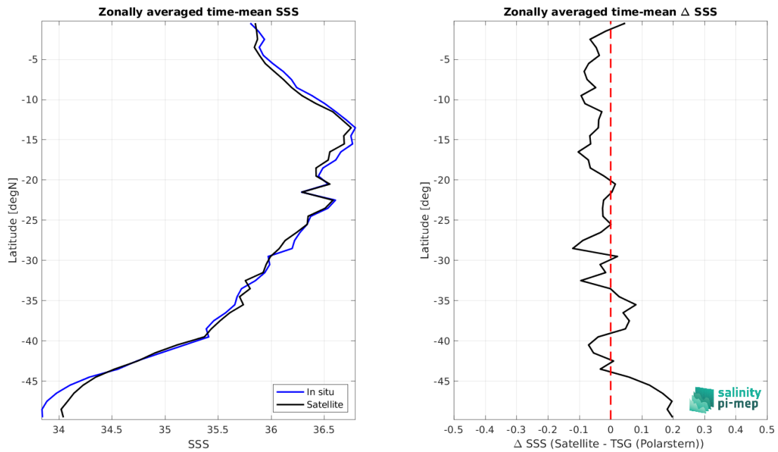
Figure 9: Left panel: Zonal mean SSS from SMAP SSS L3 v6 - Monthly (RSS) satellite product (black) and from TSG (Polarstern) (blue). Right panel: Zonal mean of \Delta SSS (Satellite - TSG (Polarstern)) for all the collected Pi-MEP match-up pairs estimated over the full satellite product period.
