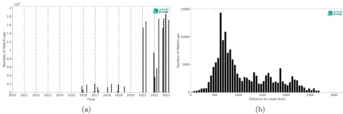
Figure 2: Number of match-ups between TSG (Polarstern) and SMAP SSS L3 v6 - Monthly (RSS) SSS as a function of time (a) and as function of the distance to coast (b) over the South Atlantic Ocean Pi-MEP region and for the full satellite product period.
