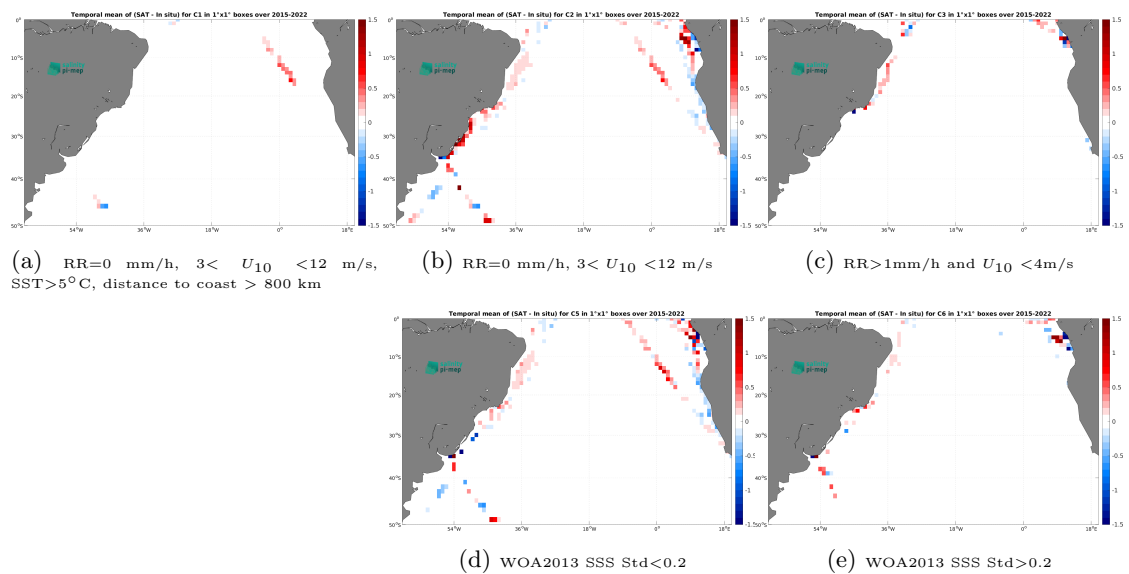
Figure 14: Temporal mean gridded over spatial boxes of size 1^\circ \times 1^\circ of \Delta SSS (SMAP SSS L3 v6 - Monthly (RSS) - TSG (LEGOS-DM)) for 5 different subdatasets corresponding to:RR=0 mm/h, 3 < U_{10} < 12 m/s, SST>5°C, distance to coast > 800 km (a), RR=0 mm/h, 3 < U_{10} < 12 m/s (b), RR>1mm/h and U_{10} < 4 m/s (c), WOA2013 SSS Std<0.2 (d), WOA2013 SSS Std>0.2 (e).
