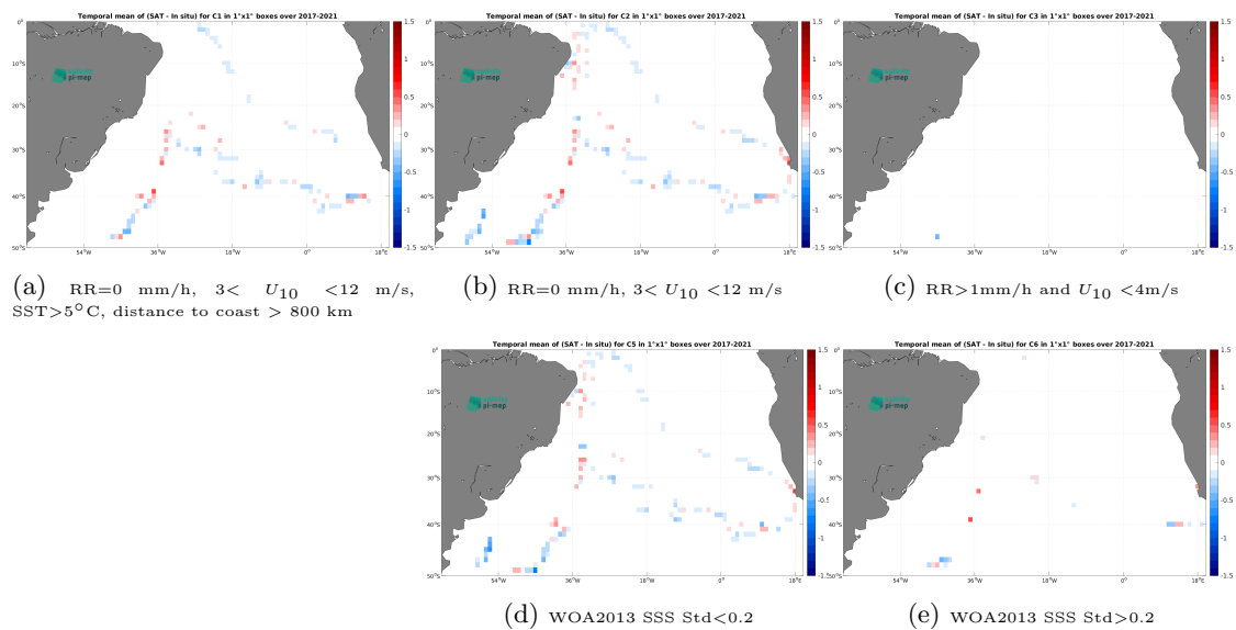
Figure 14: Temporal mean gridded over spatial boxes of size 1^\circ \times 1^\circ of \Delta\text{SSS} (SMAP SSS L3 v6 - Monthly (RSS) - TSG (GOSUD-Sailing-ship)) for 5 different subdatasets corresponding to:RR=0 mm/h, 3 < U_{10} < 12 m/s, SST >5^\circ\text{C} , distance to coast > 800 km (a), RR=0 mm/h, 3 < U_{10} < 12 m/s (b), RR >1 mm/h and U_{10} < 4 m/s (c), WOA2013 SSS Std <0.2 (d), WOA2013 SSS Std >0.2 (e).
